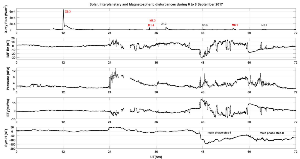
Figure 1. Variations in solar (X-ray irradiance), interplanetary (IMF B_z , solar wind pressure, and IEF _y ), and magnetospheric (SYM-H) parameters during 6 to 8 September 2017. The major solar flares during this period are labeled with the respective flare intensity. The flares highlighted in red labels are considered for this study. IMF = interplanetary magnetic field; IEF = interplanetary electric field.
