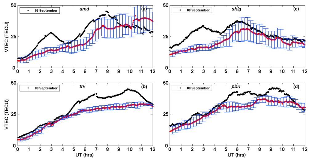
Figure 6. GPS-TEC variations as recorded at (a) amd , (b) trv , (c) shlg , and (d) pbri stations during 00:00 to 12:00 UT on 8 September 2017. Three quiet days' mean TEC along with the standard deviations for the same month are also presented in the figure.
