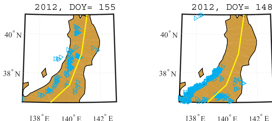
Fig. 8. An example of change of spatial distribution of lightnings in Honsyu region: (a) Day 2012 155,; (b) day 2012 148.
