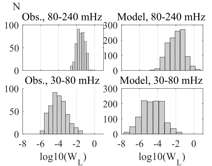
Fig. 7. The distributions of the “observational pulse index” and for the WWLLN lightning index for the nominal Pc3 (30–80 mHz) and Pc2 (80–240 mHz) frequency ranges.
