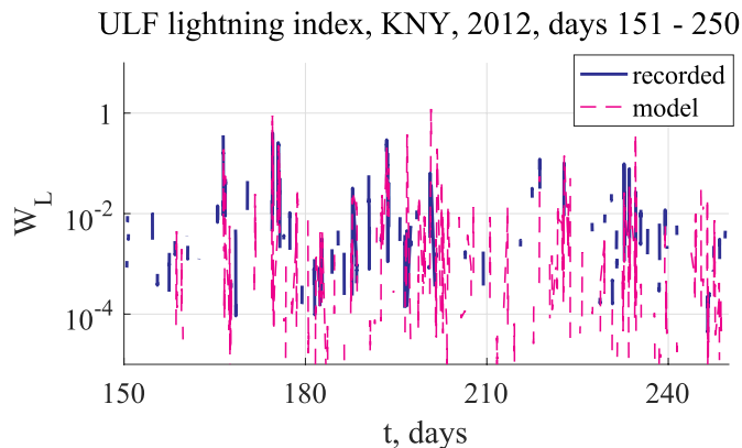
Fig. 6. Modeled and recorded values of hourly ULF lightning index at KNY for nighttime in summer of 2012.
