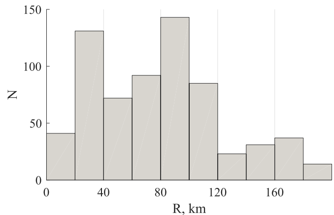
Fig. 3. Distribution of distances between strokes and the observational site.
