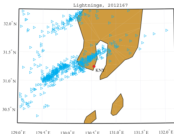
Fig. 2. Lightnings detected at WWLLN near KNY at day 2012167.
