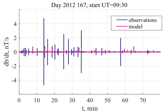
Fig. 4. Recorded and modeled variations of the magnetic field at KNY.
