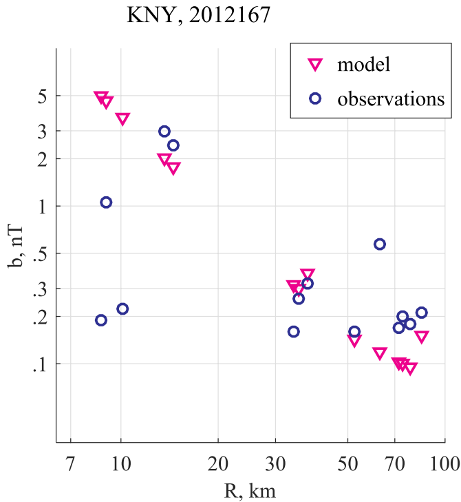
Fig. 5. Dependence of measured at KNY and model pulse amplitude on the effective distance R .
