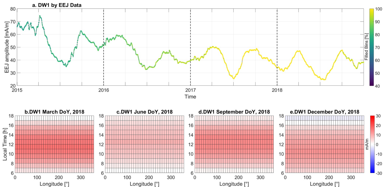
Figure 14. (a) Time series of DW1 amplitude obtained from equatorial electrojet (EEJ) data during the Swarm period ( x axis represent time with the years as labels). Vertical dashed black lines indicate the beginning of a new year. Panels b–e indicate the contribution of DW1 to the final predicted EEJ in terms of positive and negative perturbations for selected days of year from March, June, September, and December 2018, respectively.
