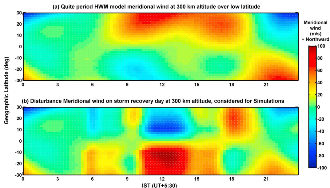
Figure 5. (a) Quiet period meridional wind based on the HWM model. (b) Disturbance meridional wind considered in the SAMI2 model during the recovery phase of the geomagnetic storm on 18 March 2015.
