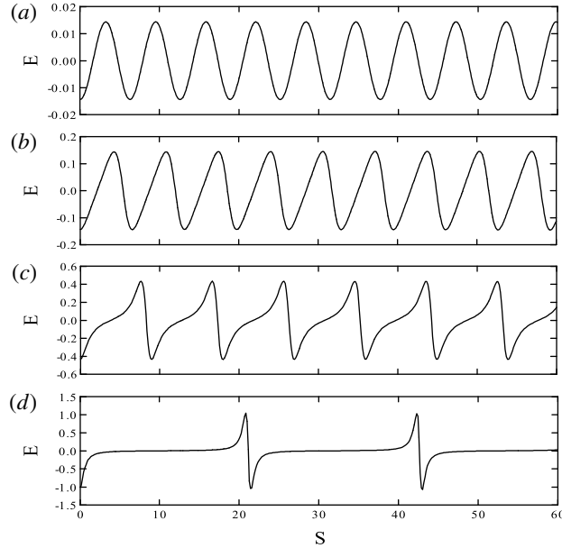
FIGURE 1. Numerical solution of the normalized electric field for the parameters M=3.5 , \theta=2^\circ , R=10.0 , \delta_c=\delta_h=0.0 , n_{ec0}/n_0=n_{pc0}/n_0=0.5 , T_c/T_h=0.0 , and E_0=(a) 0.05 (linear waveform), (b) 0.5 (sinusoidal waveform), (c) 1.5 (sawtooth waveform) and (d) 3.5 (bipolar waveform).
