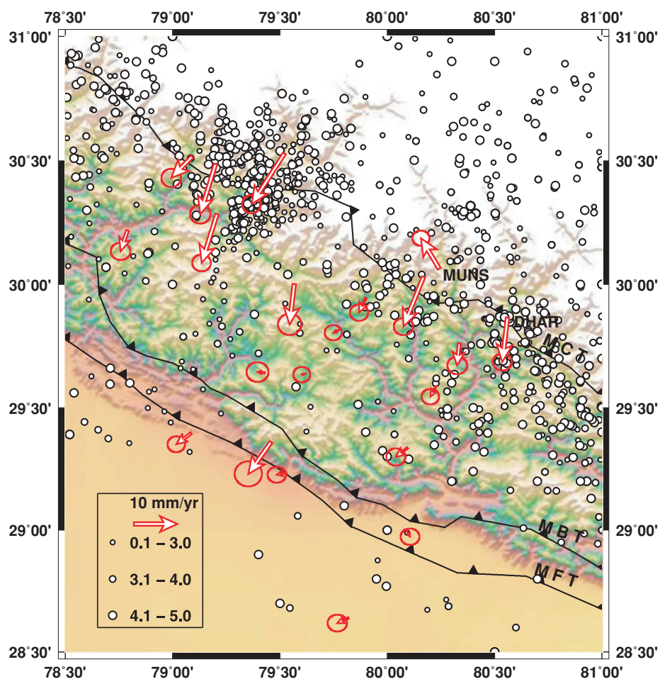
Figure 3. Estimated site velocities at our GPS stations in the Kumaun–Garhwal Himalaya with respect to the fixed Indian frame. The epicentres of the earthquakes (focal depth < 50 km) are shown as open circles (downloaded from http://www.iris.edu/data/event/eventsearch.html ). Lines with triangles denote the Main Central Thrust (MCT), Main Boundary Thrust (MBT) and Main Frontal Thrust (MFT).
