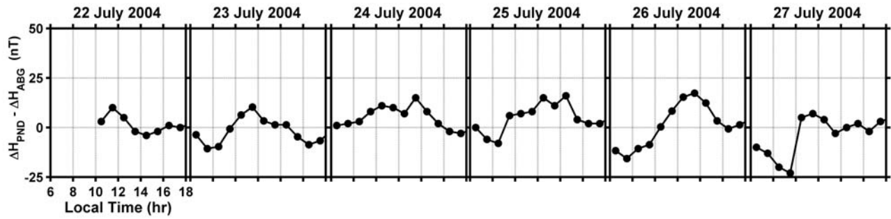
Figure 8. Daytime values of \Delta H_{\text{Pondicherry}} - \Delta H_{\text{Alibag}} during the period 22–27 July 2004 as an indicator of the latitudinal extension of the equatorial electrojet current system.
