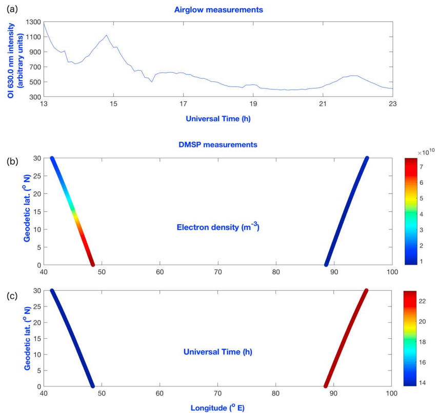
Figure 2. (a) Nocturnal variation of 630.0-nm intensity (in arbitrary units) on 3 January 2011. Defense Meteorological Satellite Program measurements of (b) the electron density at \sim 847 km over the Indian subcontinent and (c) corresponding Universal Time of measurements, respectively.
