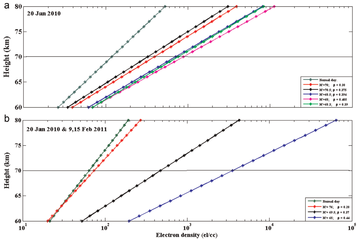
Fig. 10. (a) Comparison of electron density profiles for flares on 20th January 2010 in the noon period (10–15 LT h) and on normal day at Allahabad. (b) Comparison of the electron density profile for solar flares on 20th January 2010 and 9th and 15th February 2011 in the morning and evening periods (06–10 LT h and 15–18 LT h) with the normal day for Allahabad. (Horizontal line at 70 km is added as reference height for comparison of electron density).
