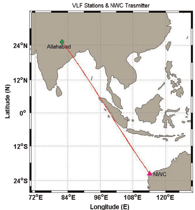
Fig. 1. Great Circle path between VLF transmitter NWC (pink triangle) and low latitude receiving stations in India Allahabad (green diamond).
