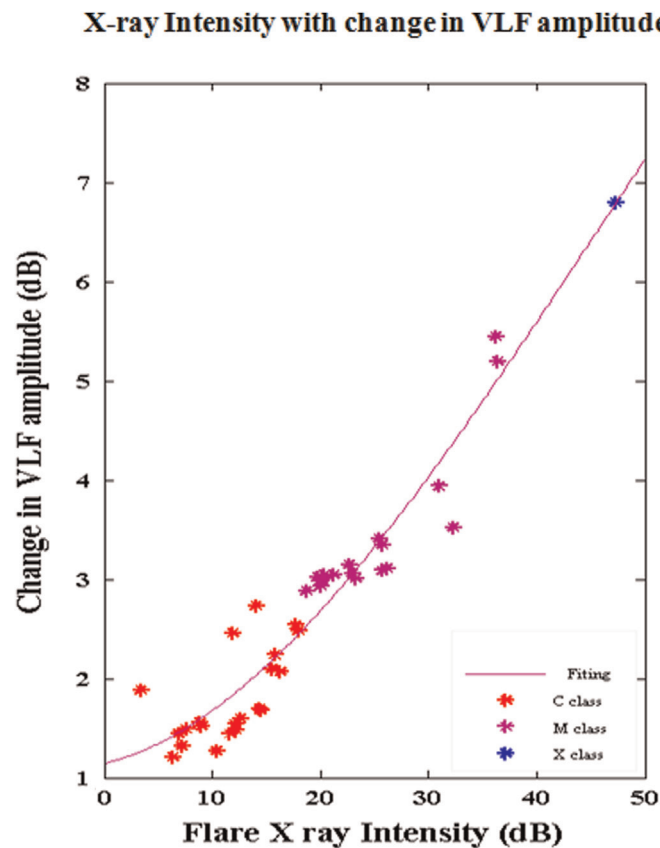
Fig. 3. Variation of change in the VLF amplitude with the solar flare intensity (dB).
