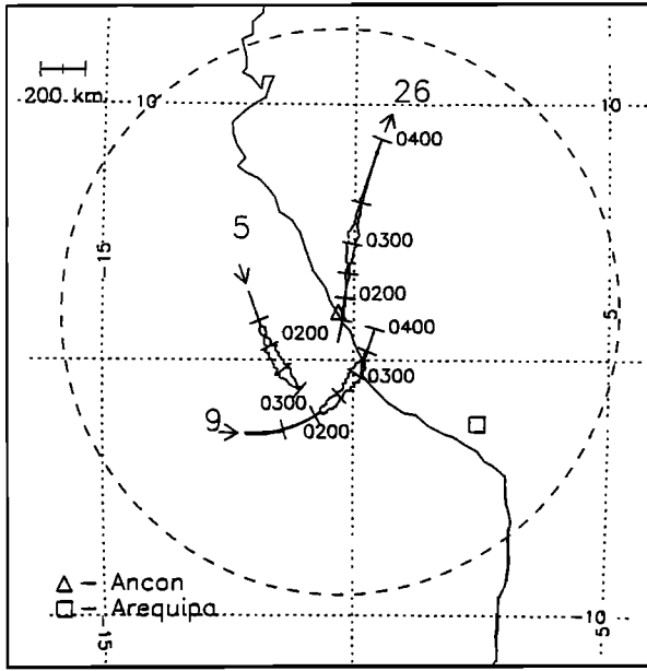
Figure 1. Tracks followed by the ionospheric penetration points, at an altitude of 350 km, of the signal paths from GPS satellites PRN 5, PRN 9, and PRN 26 to Ancon, on April 9, 1997. The time marks are in universal time (UT). Geomagnetic coordinates are given on the grid and the dashed circle represents the 350 km altitude visibility limit at Ancon for an elevation of 10^\circ . Thickness of a trace indicates strength of scintillation activity. [after Beach and Kintner, 1999 ].
