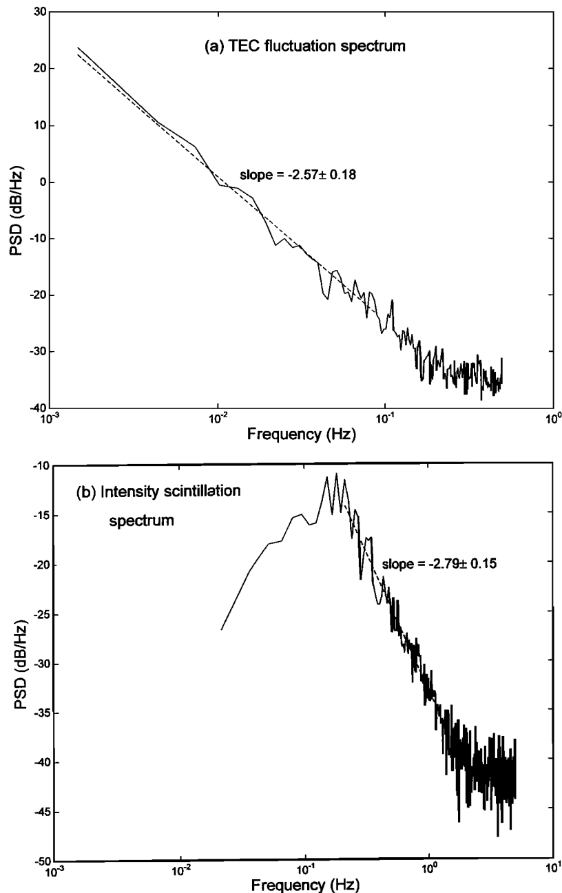
Figure 7. (a) Power spectrum of detrended TEC variations (detrend cutoff frequency is 0.0007 Hz) for the signal path from PRN 5 to Ancon, on April 9, 1997. (b) Power spectrum of detrended (detrend cutoff frequency is 0.01 Hz) 10 Hz intensity scintillation data for L1 signal from PRN 5 to Ancon during the same night.
