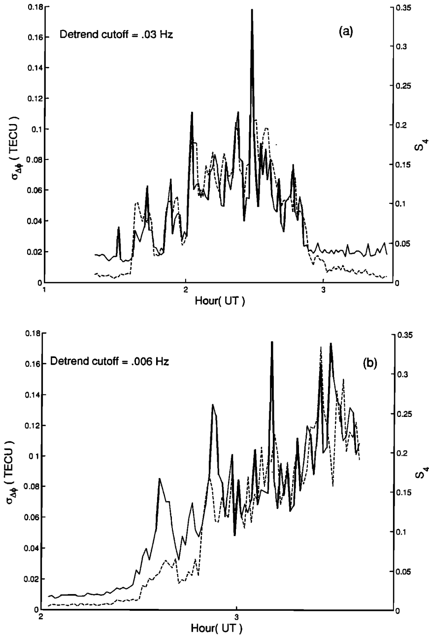
Figure 4. The \sigma_{\Delta\phi} (solid line) and S_4 (dashed line), computed from 1 Hz, dual-frequency, de-trended TEC fluctuation data and intensity scintillation data on L1, respectively, recorded at Ancon for (a) PRN 5 on April 9, 1997, and (b) PRN 26 on April 17, 1997.
