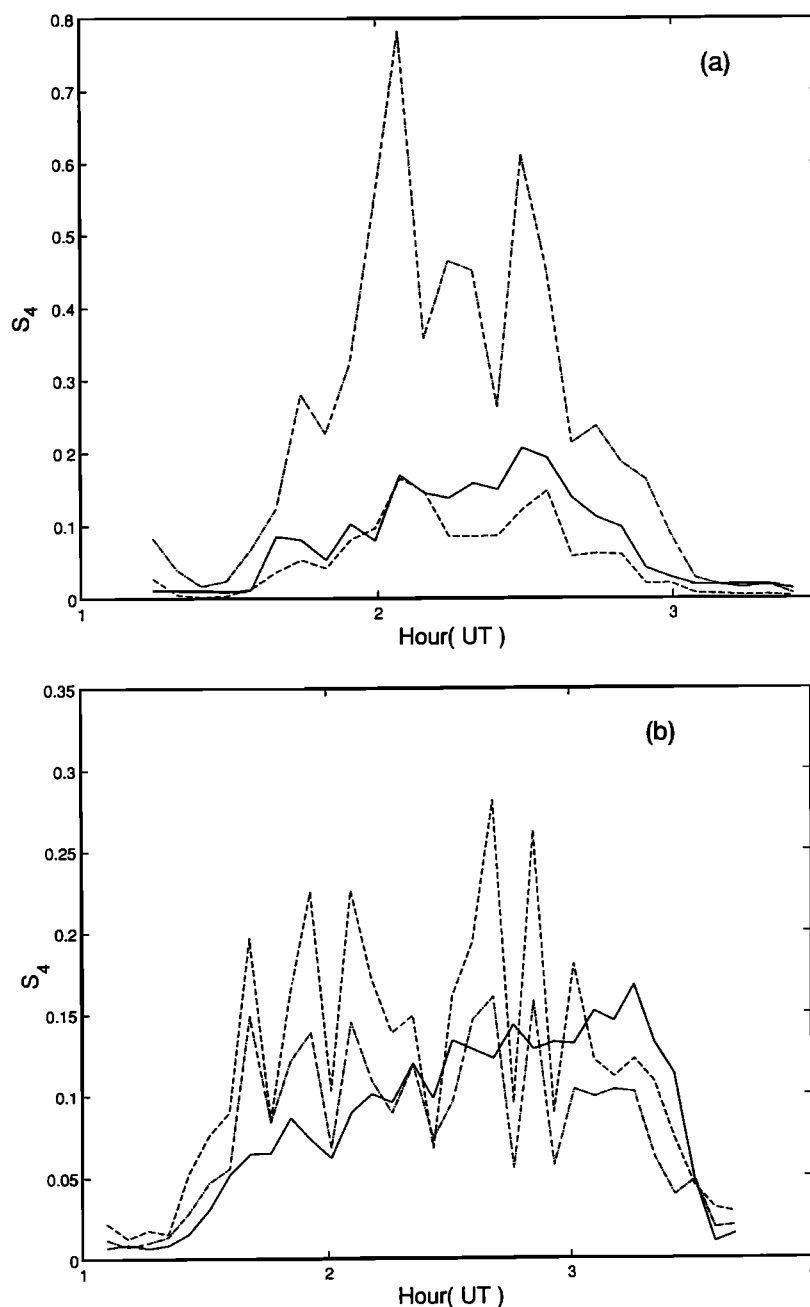
Figure 5. S_4 indices: computed from intensity scintillations on L1 (solid line), derived from DROTI ( = 1.6 \times 10^3 \nu_F^2 S_4 ) (dashed line) with DROTI in units of TECU/min 2 and \nu_F given in hertz, and derived from ROTI ( = 2.5 S_4 ) (dash-dotted line) with ROTI in units of TECU/min. Figures 5a and 5b are for the same satellite, PRN 5, for two different nights with different \nu_F : (a) April 9, 1997, \nu_F = 0.126 Hz; and (b) April 17, 1997, \nu_F = 0.053 Hz.
