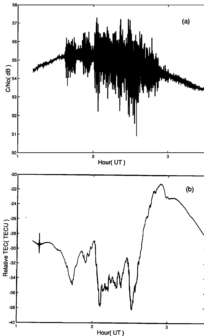
Figure 3. (a) Intensity scintillations on the L1 signal transmitted from PRN 5 to Ancon, and (b) simultaneous variations in TEC along the same signal path, measured using a dual-frequency receiver on April 9, 1997.
