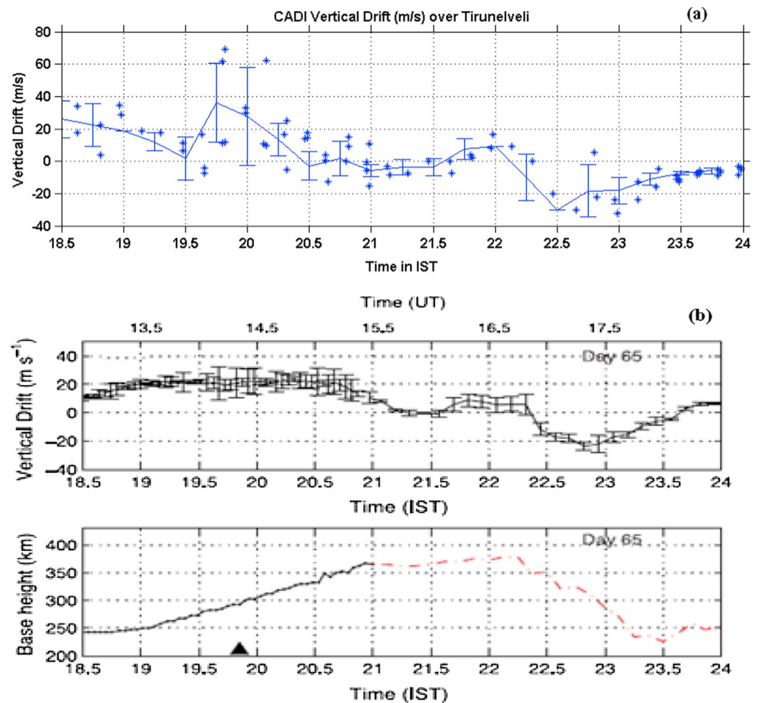
Figure 5. (a and b) The comparison of CADI drifts at Tirunelveli with that of digisonde drifts at Trivandrum on same day which is \sim 100 km away from Tirunelveli.
