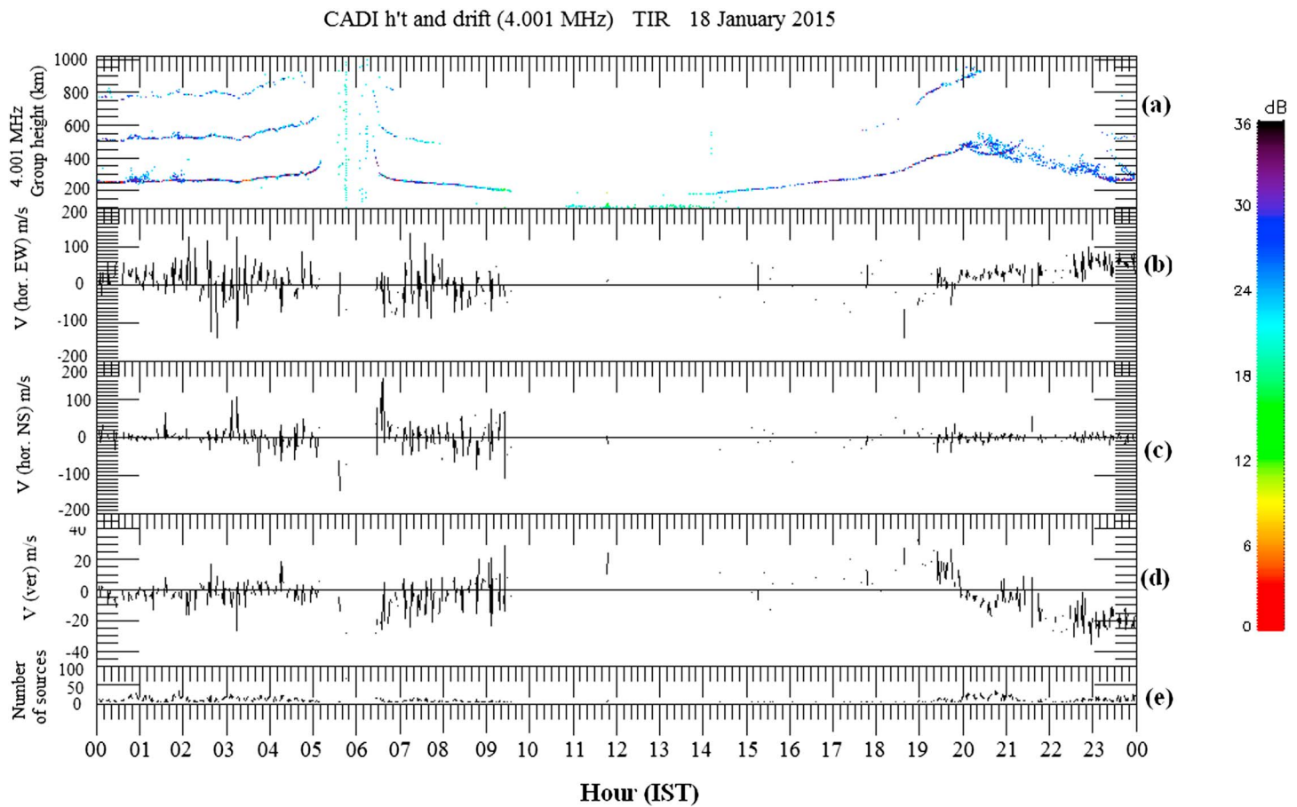
Figure 4. (The altitudinal variation of (a) typical ionization layer movement at 4 MHz and its (b) east-west, (c) north-south, (d) vertical drift (m/s), and their scattering sources.
