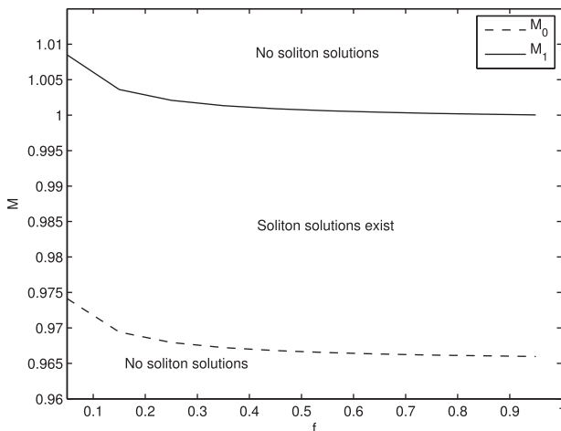
FIG. 1. Critical Mach number, M_o , and maximum Mach number, M_1 , of ion-acoustic solitons shown as a function of the normalized cool electron number density f = N_{c0}/N_0 , for \tau = 0.04 , \alpha = 0.01 , \theta = 15^\circ .
