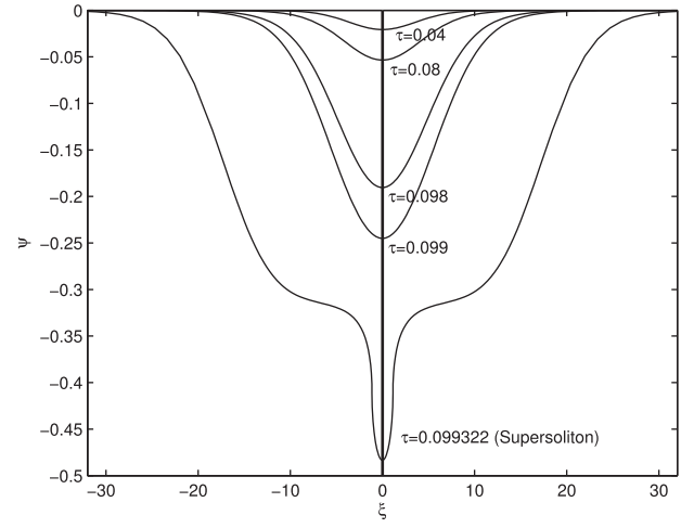
FIG. 5. The solitons and supersoliton potential \psi versus \xi for Figure 4 parameters.
