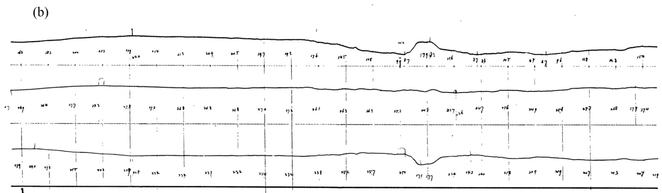
Fig. 7.2 (a) Schematic of an Eschenhagen type magnetic variometer (for details see Wienert, 1970) (b) Normal-run magnetogram recorded at Kakioka observatory on November 24, 1924. (Credit: WDC for Geomagnetism, Kyoto)
