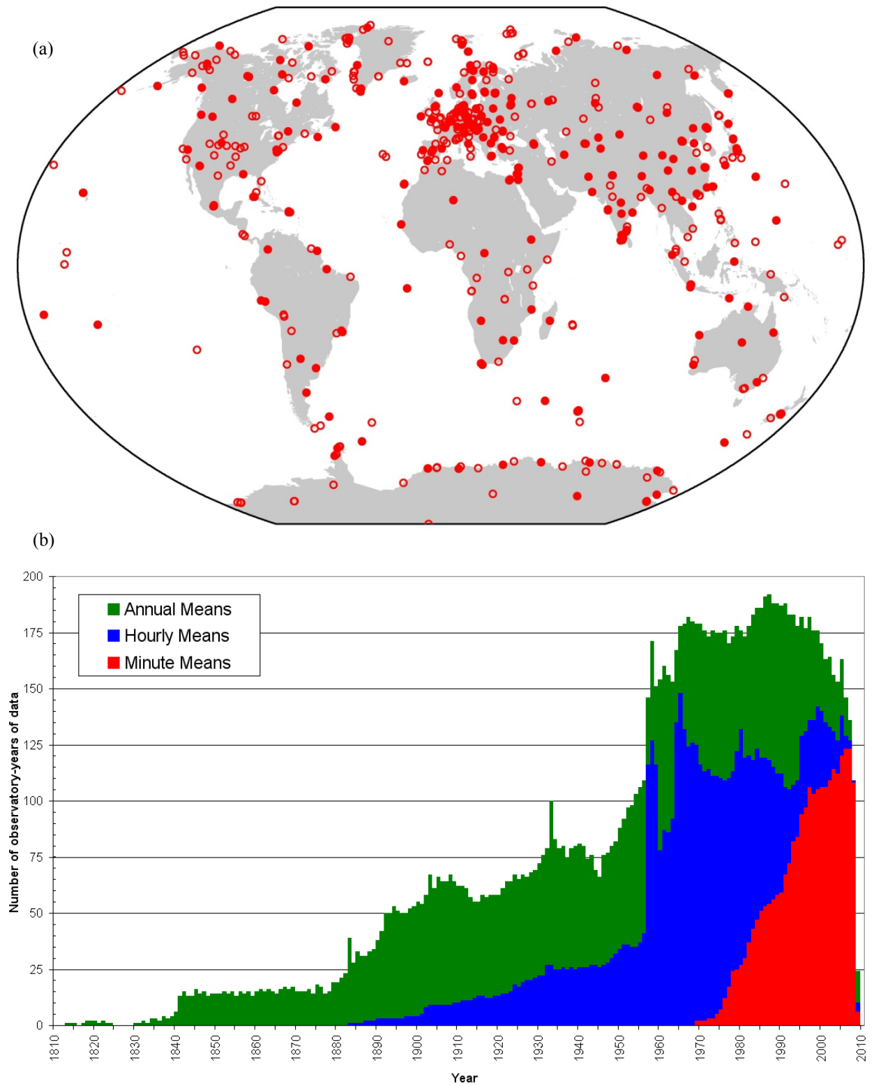
Fig. 7.7 (a) Locations of geomagnetic observatories worldwide, with data held in the Edinburgh WDC. Solid dots indicate operational observatories, open dots are sites that are currently closed (b) The number of data holdings at the World Data Centre (Edinburgh) for various time resolutions. (Copyright BGS/NERC)
