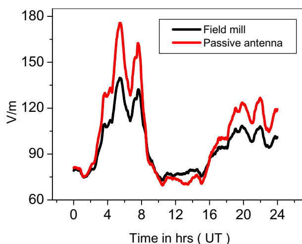
Fig.1. Comparison of the diurnal variation of potential gradient obtained on 23.2.07 from field mill and passive antenna system.
