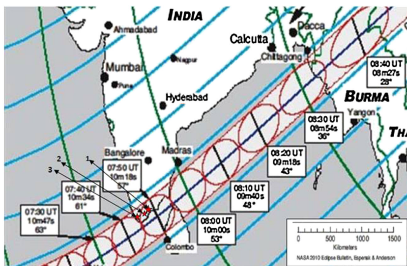
Figure 1. The track (red curves) of the solar eclipse on 15 January 2010 [Esenak and Anderson, 2010]; red stars show the observation sites (1) Tirunelveli, (2) Braemore Hills, and (3) Thiruvananthapuram where eclipse was 91%. The red ellipses and square boxes indicate the passage of the eclipse with time in UT.
