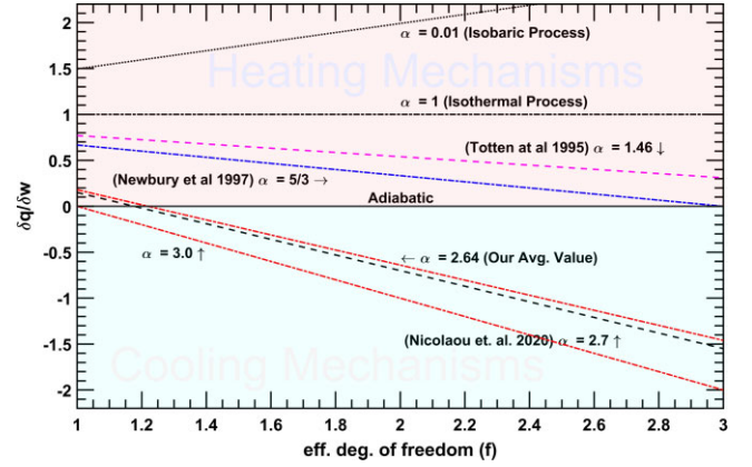
Figure 2. Relation between \frac{\delta q}{\delta w} and f for different value of \alpha . The red- and cyan-shaded regions represent the heating and cooling mechanisms. It is associated with different parameters that either supply or retain heat from the expanding plasma region. In plot, we show variation for different \alpha values, such as; 2.64 (average value in this work), 2.7 (Nicolaou et al. 2020), 5/3 (Newbury, Russell & Lindsay 1997), 1.46 (Totten, Freeman & Arya 1995), \alpha = 0.1 (isobaric process), \alpha = 1 (isothermal process), and \alpha = 3 (highly superadiabatic), respectively.
