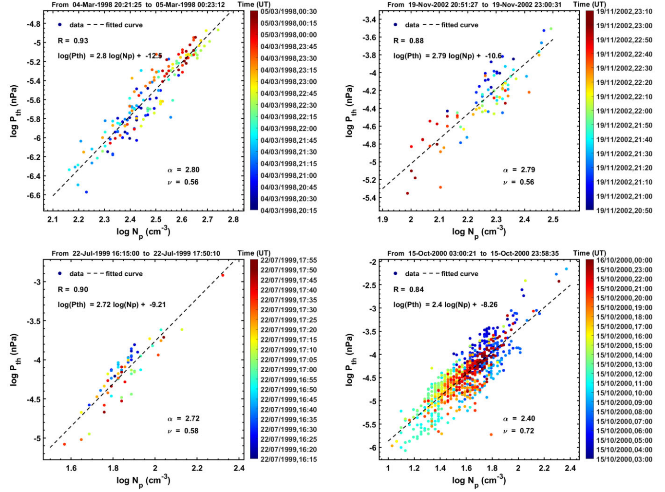
Figure 1. Variation of \log P_{th} versus \log N_p . The coloured circles represent data points (time evolution) and black-dashed line gives linear fitting value.
