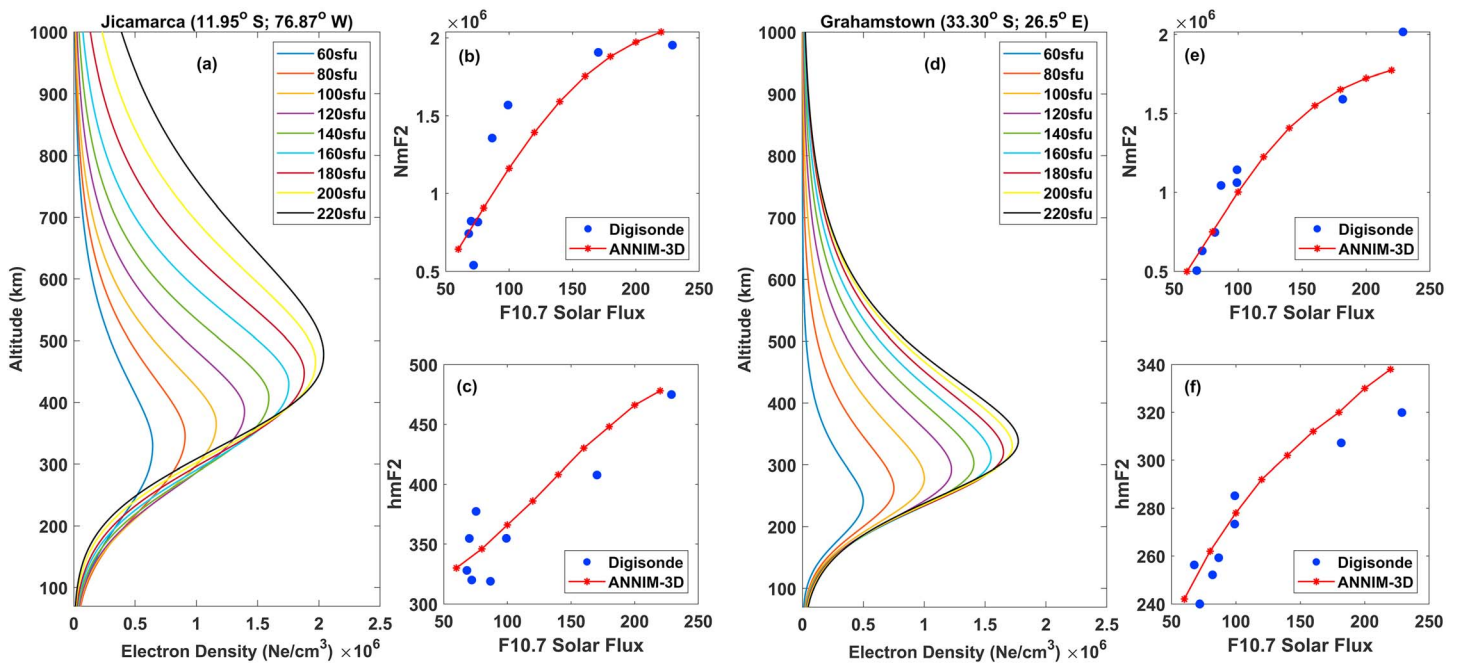
Figure 4. Vertical electron density profiles for 12 local time under March equinox conditions, simulated by ANNIM-3D for varying F_{10.7} solar flux inputs and comparisons of N_mF2/h_mF2 with collocated Digisonde observations at an equatorial location, Jicamarca (a–c) and a midlatitude station, Grahamstown (d–f). ANNIM-3D = artificial neural network-based global three-dimensional ionospheric model.
