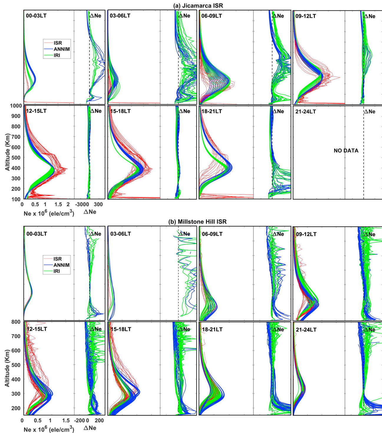
Figure 5. Comparison of artificial neural network-based global three-dimensional ionospheric model-predicted electron density profiles (blue curves) with ground based ISR profiles (red curves) at Jicamarca (Figure 5a) and Millstone Hill (Figure 5b) during March 2013. The IRI 2016-predicted (green curves) profiles have also shown for comparison. The percentage of deviations in the model predictions with respect to ISR observations ( \Delta Ne \% = ((\text{model Ne} - \text{ISR Ne}) / \text{ISR Ne}) \times 100 ) were shown in the right-hand side insets in each panel using the same color scheme. ISR = incoherent scatter radar.
