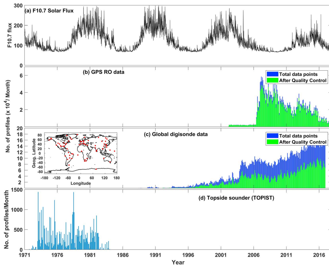
Figure 1. Quantum of data assimilated in artificial neural network-based global three-dimensional ionospheric model. (a) The daily variation of F10.7 solar flux from 1971 to 2016. (b) Number of global positioning system-radio occultation (GPS-RO) profiles per month from CHAMP, GRACE, and FORMOSAT-3/COSMIC together. (c) Number of bottomside profiles per month from GIRO-Digisonde network. The locations of the Digisonde stations considered in the study can be seen in the inset of Figure 1c. The blue bars (in Figures 1b and 1c) indicate the total number of electron density profiles per month, and the green bars represent the electron density profiles after the quality control measures. (d) The total number of electron density profiles per month from the topside sounders onboard International Satellites for Ionospheric Studies satellites.
