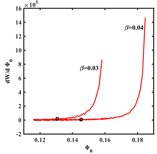
FIG. 7. Variation of slope of the W - \Phi_0 with \Phi_0 .
