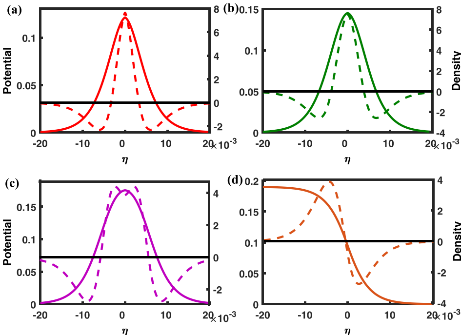
FIG. 4. Potential and \Delta n profiles for SWs and DL; (a) and (b) RSW, (c) transitional RSW, and (d) DL.
