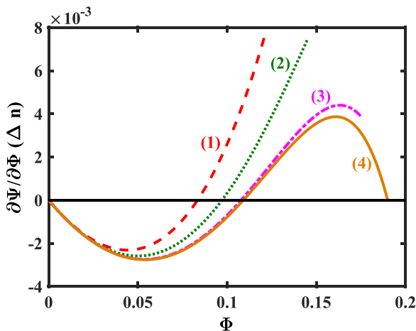
FIG. 2. Variation of \Delta n Vs \Phi ; curves (1) and (2) RSW, (3) transitional RSW, and (4) DL.
