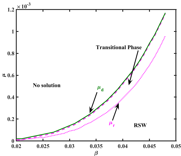
FIG. 9. Regime of SWs and DLs.
