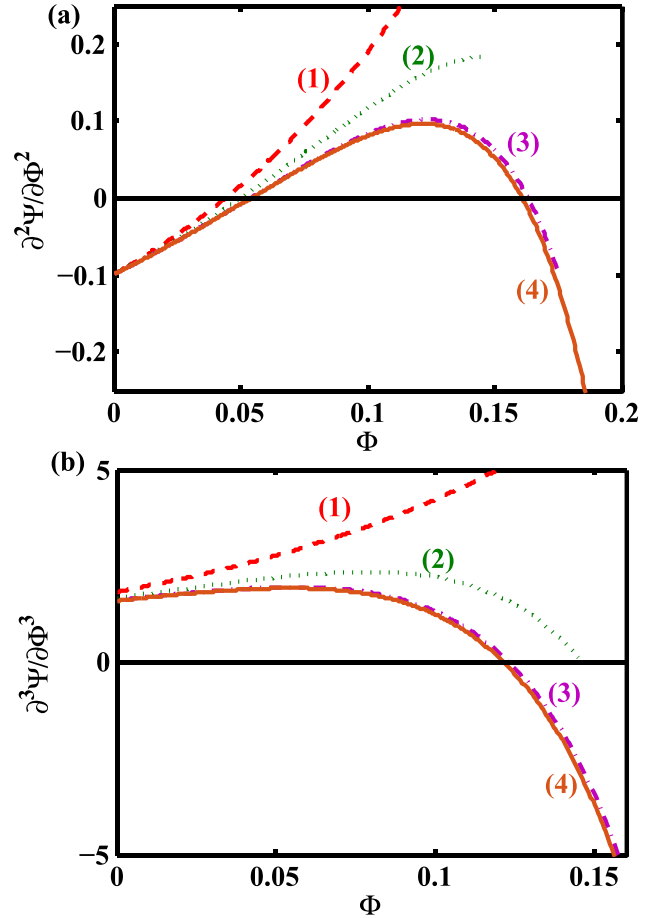
FIG. 3. (a) Variation of \frac{\partial^2\Psi}{\partial\Phi^2} Vs \Phi and (b) \frac{\partial^3\Psi}{\partial\Phi^3} Vs \Phi ; curves (1) and (2) RSW, (3) transitional RSW, and (4) DL.
