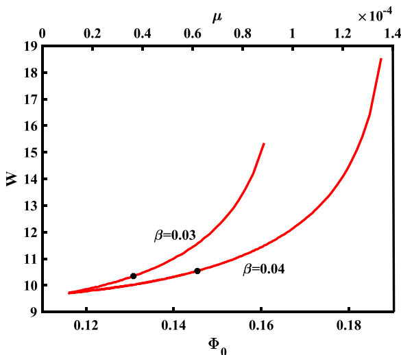
FIG. 6. Variation of W with \Phi_0 with \mu .
