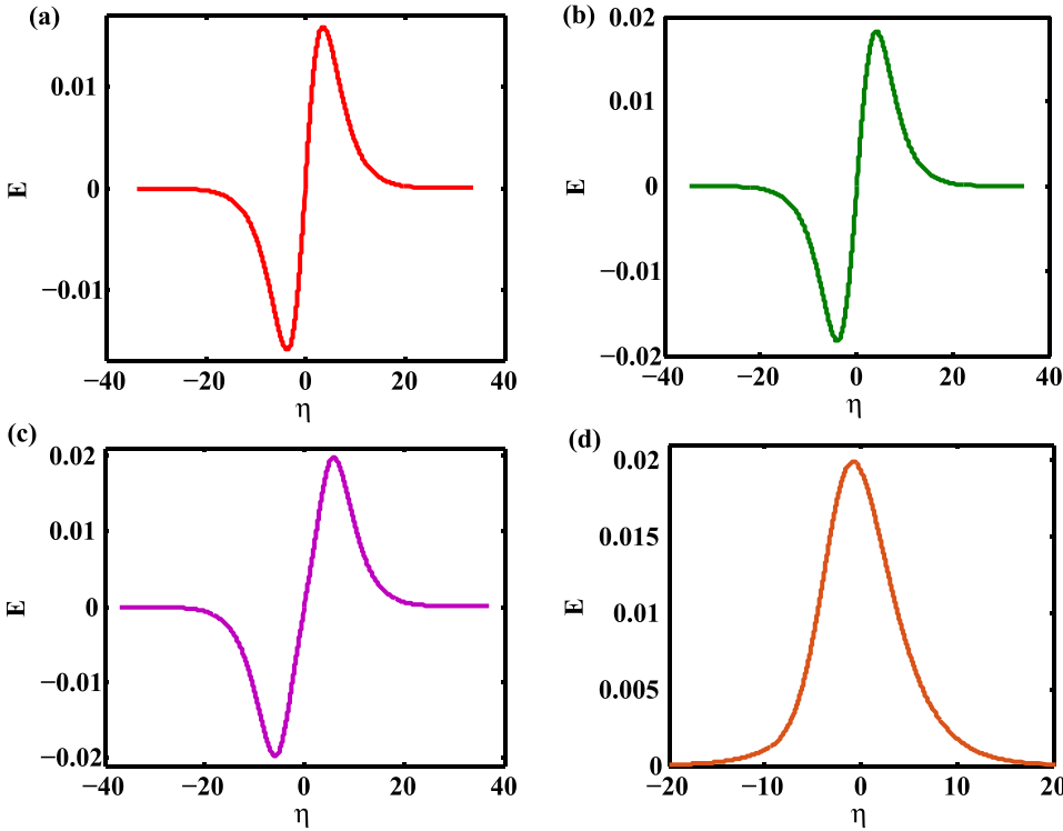
FIG. 5. Electric Field profile for SWs and DL; (a) and (b) RSW, (c) transitional RSW, and (d) DL.
