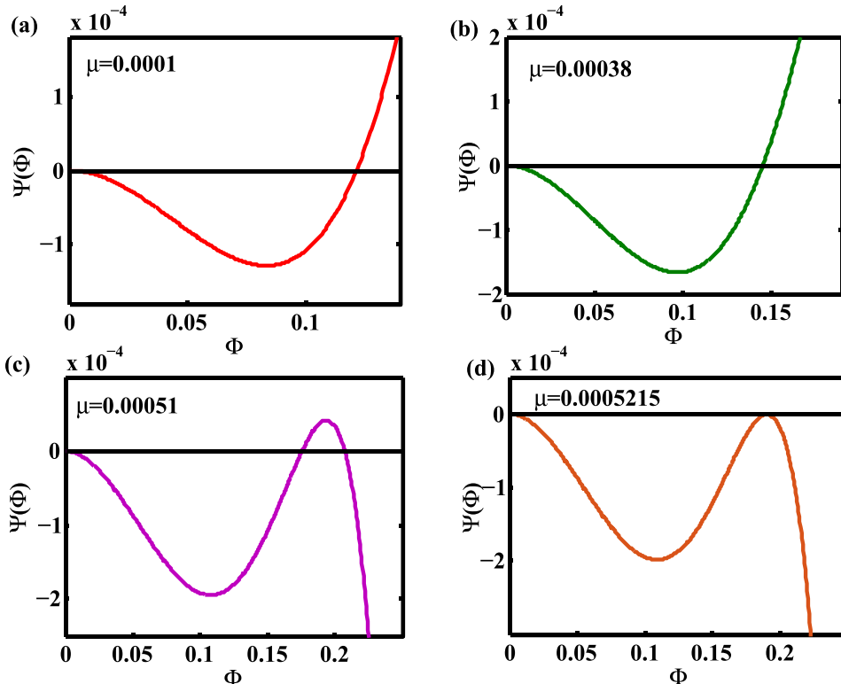
FIG. 1. Sagdeev pseudopotential profiles; curves (a) and (b) RSW, (c) transitional RSW, and (d) DL.
