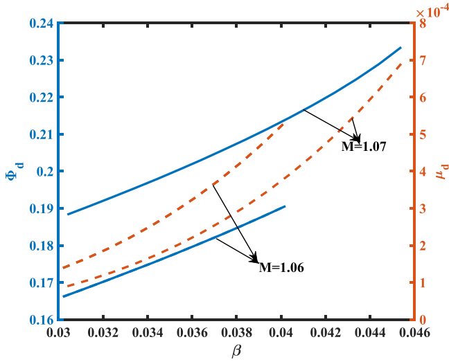
FIG. 8. Variation of \mu_d and \Phi_d with \beta .
