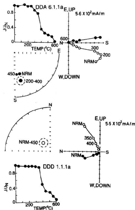
Fig. 3. Thermal demagnetization results of two specimens from region 1. Stereonetic projections and intensity decay (left), Zijderveld diagrams (right). On the stereonet, solid (open) circles are projections on the lower (upper) hemisphere. Dashed outline indicates directions in the temperature intervals shown and have no statistical significance. On the Zijderveld diagrams, open circles are projections of the end points of demagnetization vector on a north-south vertical plane, solid circles on the horizontal plane. J/J_N denotes normalized intensity.
