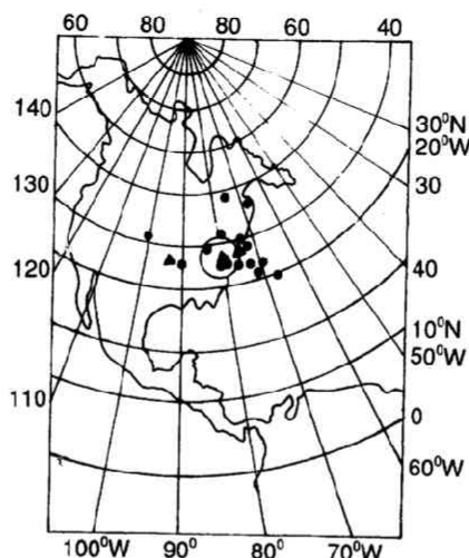
Fig. 9. Pole positions from the Deccan lava flows (circles) and dykes (triangles). The pole from the present study is plotted with its A_{95} confidence circle (see Table 3).
