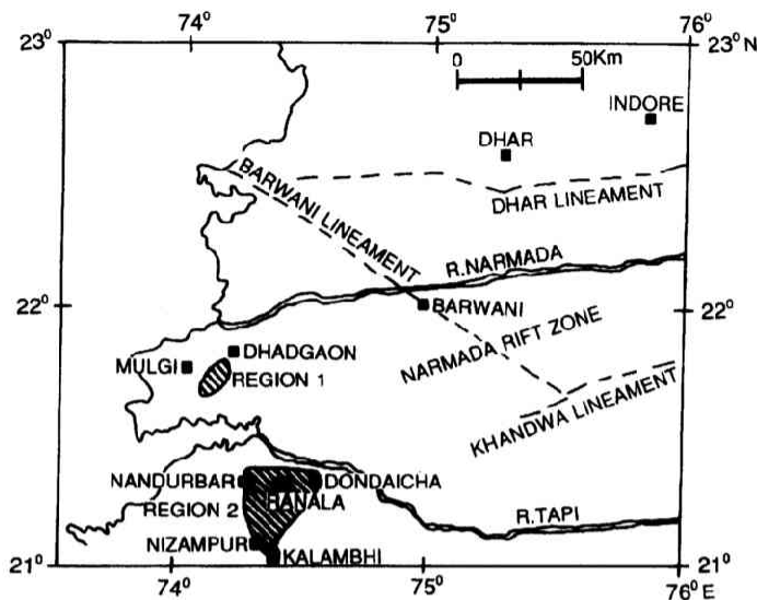
Fig. 2. Sampling localities of Regions 1 and 2 in the Narmada-Tapti tectonic belt.
