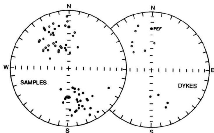
Fig. 7. Characteristic sample and site mean directions. Equal area plot. Symbols as in Fig. 3.
