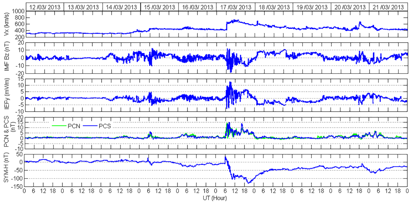
Figure 2. Variations of the solar wind speed ( V_x ), interplanetary magnetic field ( IMF B_z ), Interplanetary electric field ( IEFY ), Polar cap indices (PCN and PCS), and SYM-H index on 12–21 March 2013.
