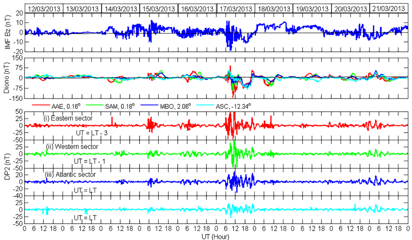
Figure 3. Variations of IMF B_z along with Diono and DP2 over Addis Ababa (red) in the Eastern sector, Samogossoini (green) in the Western sector, Mbour (blue), and Ascension Island (cyan) in the Atlantic sector from 12 to 21 March 2013.
