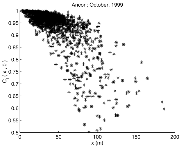
Figure 3. Spatial correlation function C_I(x, 0) of intensity scintillation pattern in the plane of the receiver, versus spatial lag x , for UHF scintillations recorded at Ancon during October, 1999.
