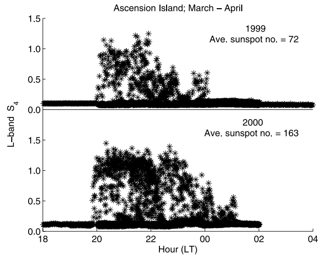
Figure 4. Distribution of L-band S_4 -indices obtained at Ascension Island, as a function of local time, for 9 nights of March–April, 1999 (top panel) and 12 nights of March–April, 2000 (bottom panel). The average values of sunspot numbers for the two periods are given in the figure.
