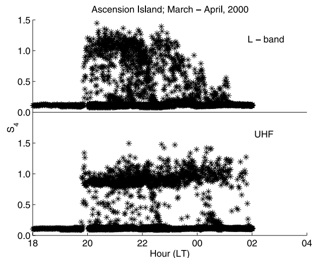
Figure 5. Comparison of the distributions of L-band (top panel) and UHF (bottom panel) S_4 -indices obtained at Ascension Island, as a function of local time, during March–April, 2000.
