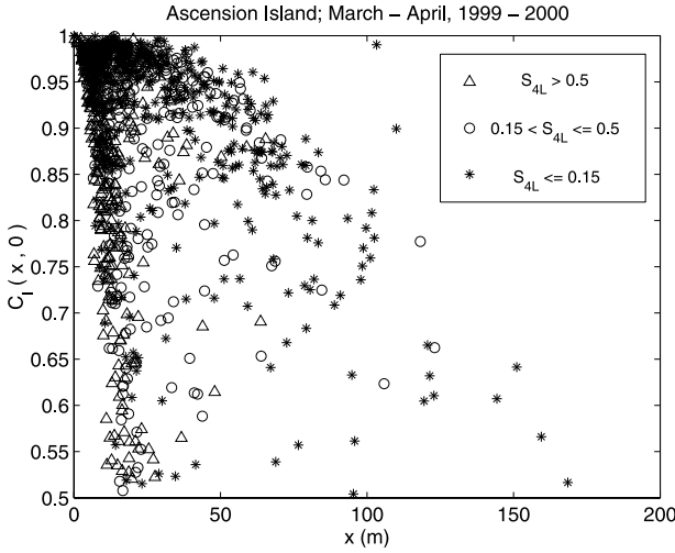
Figure 1. Spatial correlation function C_I(x, 0) of intensity scintillation pattern in the plane of the receiver, versus spatial lag x , for UHF scintillations recorded at Ascension Island during March–April, 1999 and 2000. The points are assigned different symbols corresponding to different levels of L-band scintillations recorded simultaneously with the UHF scintillations.
