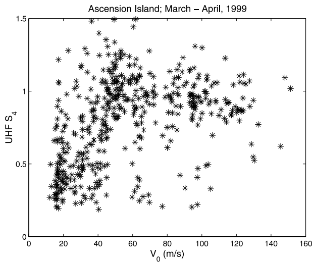
Figure 8. Variation of UHF S_4 -indices with the magnetic eastward drift, V_0 , of the ground scintillation pattern obtained at Ascension Island during March–April, 1999.
