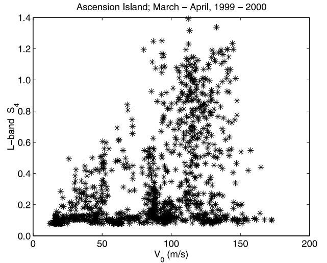
Figure 7. Variation of L-band S_4 -indices with the magnetic eastward drift, V_0 , of the UHF ground scintillation pattern obtained at Ascension Island during March–April, 1999 and 2000.
