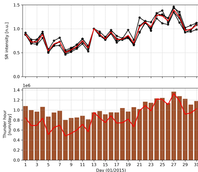
Figure 7. Comparison of normalized daily average SR intensity records (in normalized units, reference day: 13 January) from four stations (top) with the total daily numbers of Earth Networks Thunder Hours (bottom) in the 1–31 January 2015 time interval. In the top subplot black curves correspond to different SR stations while the red curve there shows the average of all records. The scaled version of the latter curve is also shown on the bottom plot. The correlation between the average SR intensity curve and thunder hours is 0.9.
