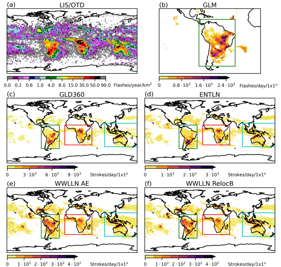
Figure 2. Lightning activity in the 13–31 January 2019 period as seen by different lightning detection methods (except in panel (a) which shows climatological lightning activity for January based on HRMC LIS/OTD observations (Cecil, 2006)). Green (South America), red (Africa) and blue (Maritime Continent) rectangles show those parts of the lightning maps for which stroke/flash numbers and thunder hours are summarized in the chimney-by-chimney analysis (Figures 5, 6b, and 6c). Note that the upper limits of the color scales are different for the different lightning detection methods.
