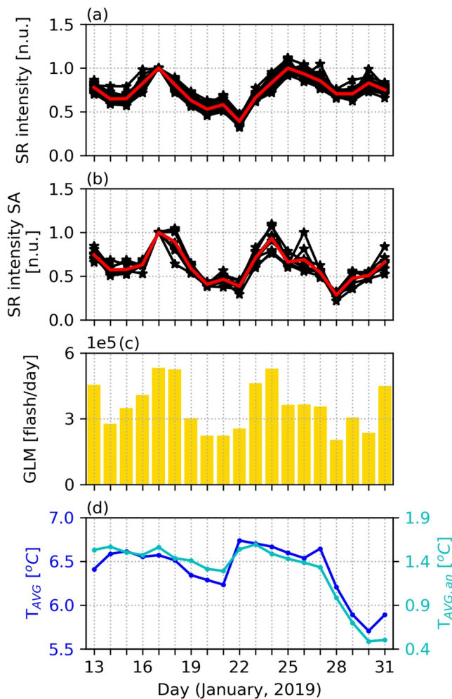
Figure 6. Comparison of (a) normalized daily average SR intensity records (in normalized units) with (b) the normalized average SR intensity records of South America (in normalized units), (c) daily flash rates provided by the GLM instrument and (d) daily global mean land surface temperatures ( T_{AVG} ) and temperature anomalies ( T_{AVG,an} ). GLM-detected lightning flashes had been summarized within the green rectangle (representing South America) marked in Figure 2.
