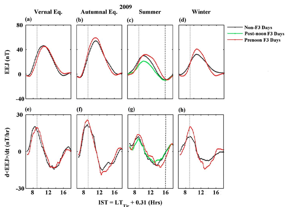
Figure 9. (a–h) Comparison of equatorial electrojet (EEJ) on F_3 and non- F_3 days for 2009 as a function of IST. The green curve in Figure 9g represents the days with F_3 layer during the postnoon hours only. The vertical black dotted line shows the time of maximum occurrence of the F_3 layer for each season. The vertical dash-dotted line represents the time of maximum occurrence for the postnoon F_3 layers during the summer of 2009. Figures 9a–9d show the 15 min averaged EEJ strength for each season and Figures 9e–9h represent the corresponding rate of change in EEJ.
