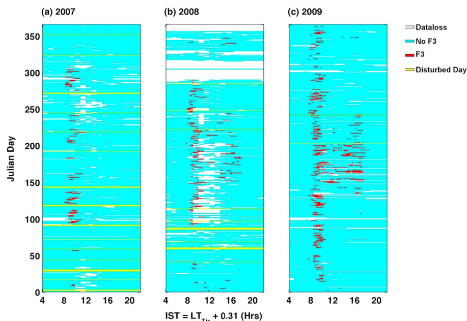
Figure 3. Occurrence of F_3 layer (red) as a function of IST during (a) 2007, (b) 2008, and (c) 2009. Disturbed days ( A_p \geq 18 ) and data loss are shown by yellow and white colors, respectively.
