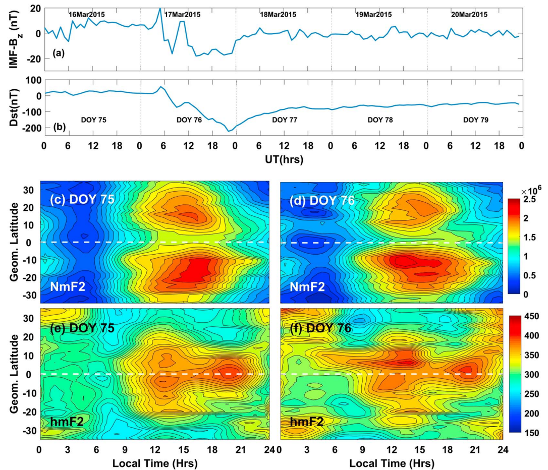
Figure 2. (a) IMF-B z and (b) Dst index from Days 75 to 79 (16–20 March 2015). Local time and dip latitudinal variation of zonal mean N m F 2 (c and d) and h m F 2 (e and f) during quiet (DOY 75; 16 March 2015) and disturbed (DOY 76; 17 March 2015) geomagnetic conditions as predicted by artificial neural network-based ionospheric model. The horizontal dashed lines represent the dip equator. DOY = day of the year.
