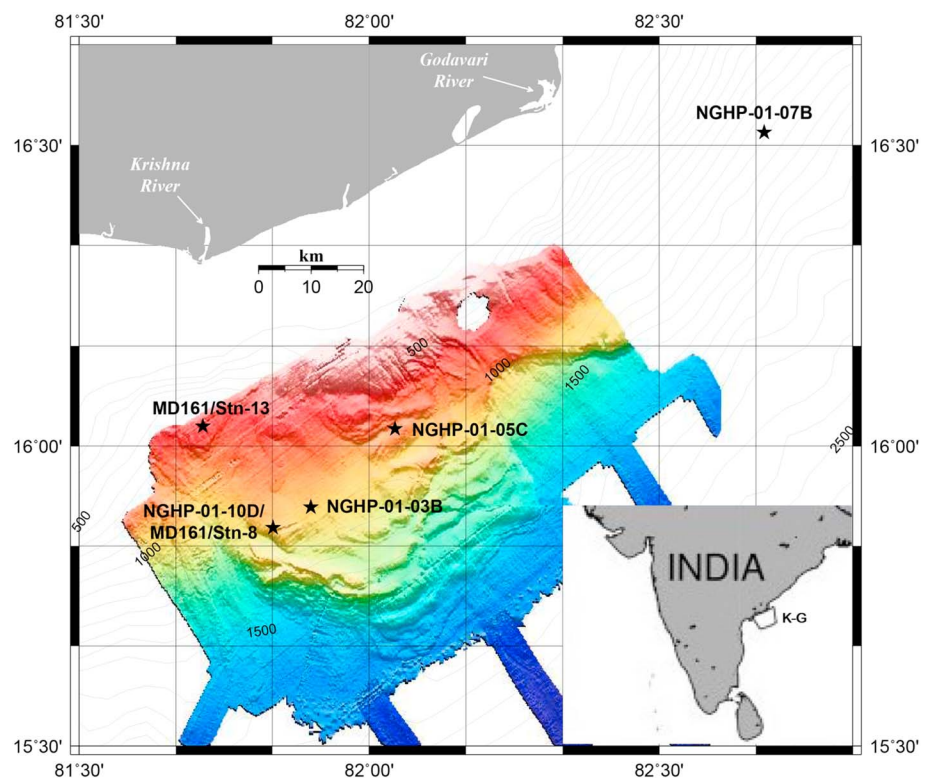
Figure 1. Location map of sediment cores NGHP-01-10D, NGHP-01-03B, NGHP-01-05C, NGHP-01-07B, MD161/Stn-8, and MD161/Stn-13 in the Krishna-Godavari basin, Bay of Bengal.
