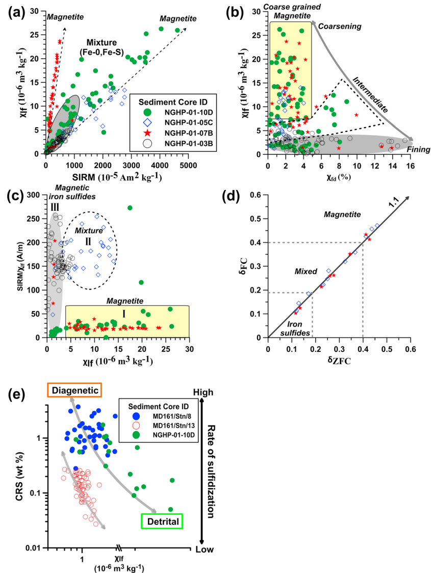
Figure 9. (a–c) Scatterplots of magnetic parameters ( \chi , saturation isothermal remanent magnetization (SIRM), \chi_{fd}\% , SIRM/ \chi , and anhysteretic remanent magnetization (ARM)/SIRM) for cores NGHP-01-10D, NGHP-01-03B, NGHP-01-05C, and NGHP-01-07B. (d) \delta_{FC} versus \delta_{ZFC} derived from low-temperature measurements (Moskowitz et al., 1993) for cores NGHP-01-05C and NGHP-01-07B. (e) Plot of chromium reducible sulfur (CRS) versus \chi_{lf} for sediment cores NGHP-01-10D, MD161/Stn-8, and MD161/Stn-13. Note that gray arrows in the scatter plots are used to highlight trends. Magnetic and CRS data for sediment cores NGHP-01-10D, MD161/Stn-8, and MD161/Stn-13 are from Badesab et al. (2017) and Peketi et al. (2012, 2015).
