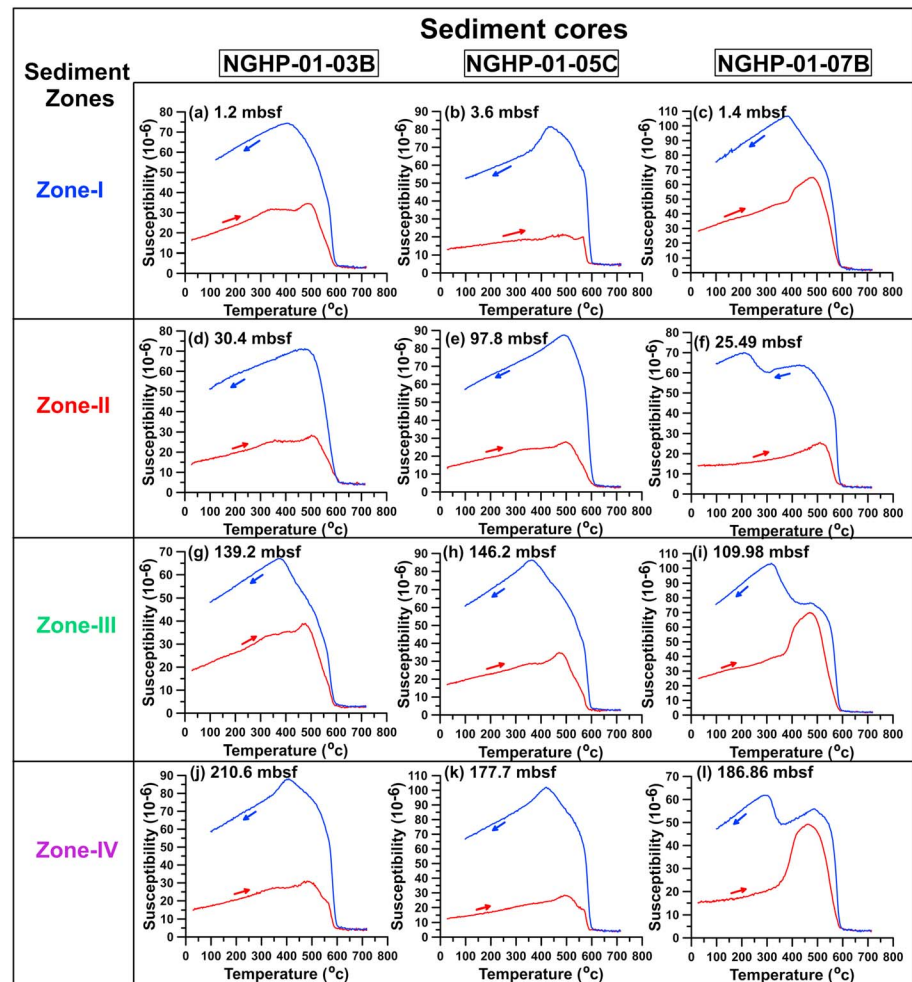
Figure 4. Temperature dependence of magnetic susceptibility ( \chi - T ) for selected representative samples from the four sediment zones of the three studied sediment cores NGHP-01-03B, NGHP-01-05C, and NGHP-01-07B. Solid red lines indicate heating curves, and blue lines indicate cooling curves.
