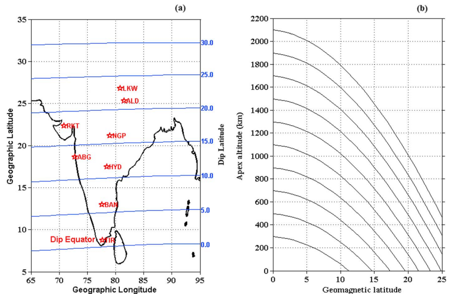
Figure 1. (a) The location of stations used in the present analysis and (b) the latitude-altitude variation of field line geometry.
