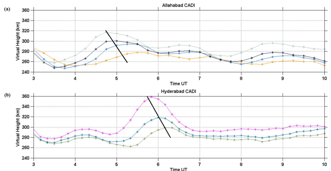
Figure 7. The temporal variation of isodensity plot at (a) Allahabad (5–8 MHz) and (b) Hyderabad (5–7 MHz) stations, respectively. The black line indicates variation of phase velocity.
