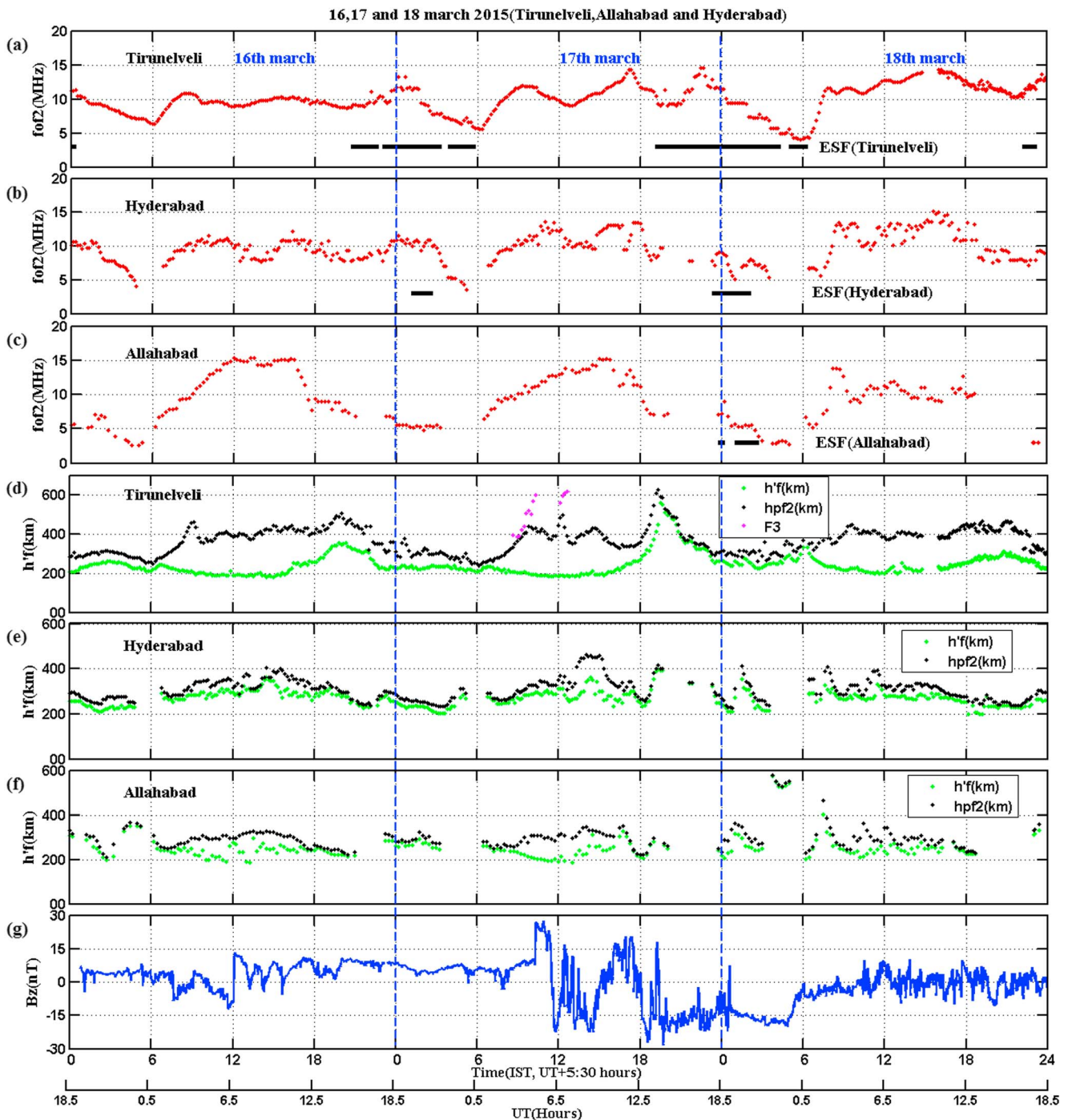
Figure 3. The temporal variations of ionospheric F region density in terms of f_oF_2 in MHz (red) for (a) Tirunelveli, (b) Hyderabad, and (c) Allahabad. h'F in km (green) and h_pF_2 in km (peak height) (black) for (d) Tirunelveli, (e) Hyderabad, and (f) Allahabad, respectively, during 16–18 March 2015. F_3 layer (magenta) is also visible in Figure 3d. (g) These figures are supported by B_z for comparison.
