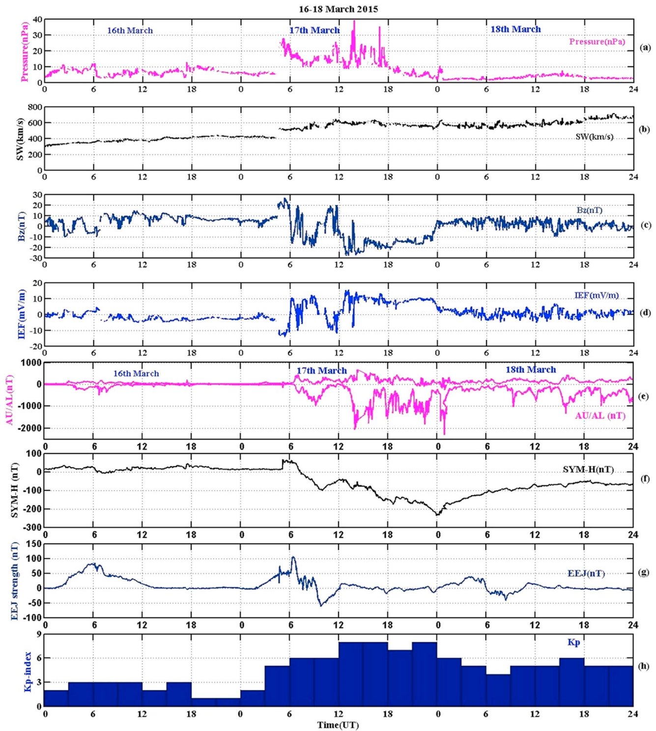
Figure 2. Temporal variations in (a) solar wind pressure, (b) speed, (c) IMF B_z , and (d) IEF in GSM coordinates for the period of 16 to 18 March 2015 and geomagnetic indices, namely, (e) AE (AU/AL) index, (f) SYM-H, (g) EEJ strength, and (h) Kp index for the same period are shown.
