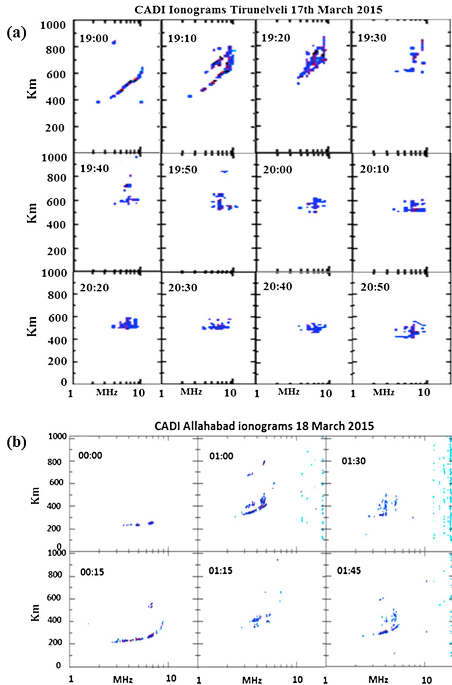
Figure 5. Ionogram images of ESF over (a) Tirunelveli and (b) Allahabad as obtained from CADI on 17–18 March 2015 (night).
