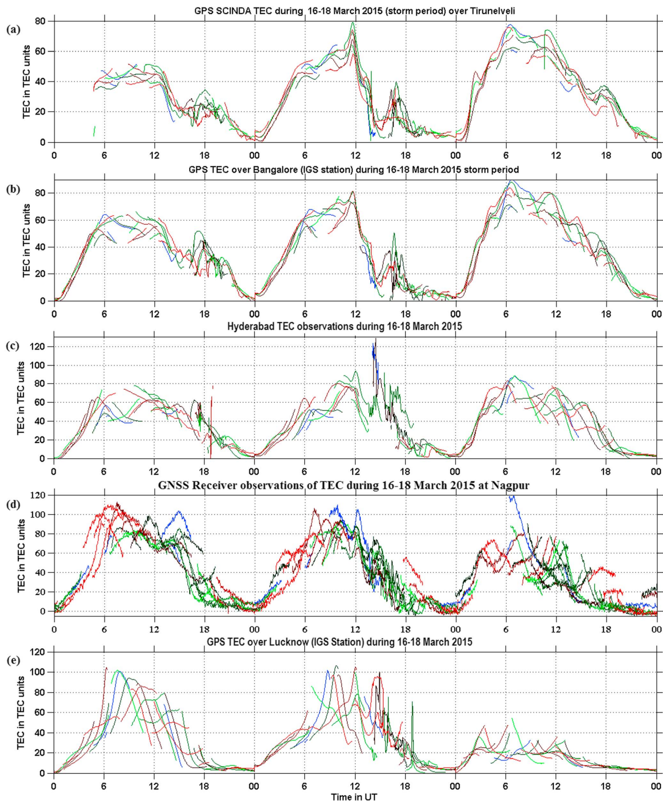
Figure 9. Temporal variations of GPS TEC over (a) Tirunelveli, (b) Bangalore, (c) Hyderabad, (d) Nagpur, and (e) Lucknow during 16–18 March 2015.
