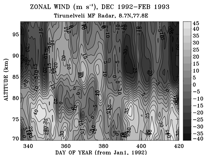
Fig. 1. Height–time cross section of mesospheric daily mean zonal wind velocity observed at Tirunelveli at 8.7°N over the period from December 1992 to February 1993.
