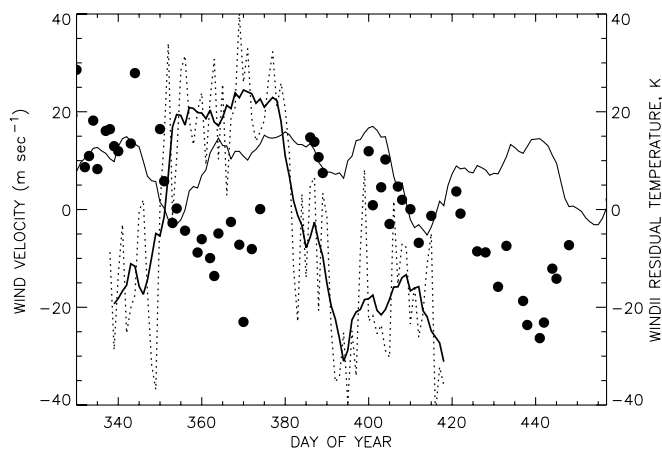
Fig. 5. WINDII temperatures and zonal wind velocities at 86 km for the period from December 1992 to March 1993. The thin solid line gives the zonal wind velocities at 87.5 km altitude and at 55°N (meteor radar at Juliusruh), the dotted line gives the MFR zonal wind velocities at 86 km, along with the 7-day smoothed data (thick solid line) and the WINDII daily zonal mean temperatures at 86 km averaged over the latitude range of 5°–15°N and centred at 10°N (solid circles).
