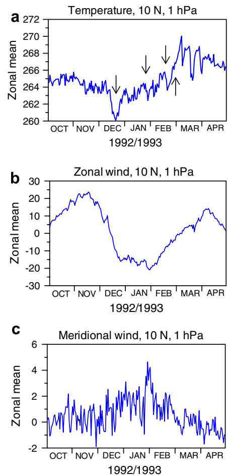
Fig. 7. The UKMO assimilated data for the periods of October 1992 to April 1993 at 10 N and 1 hPa pressure level ( \sim 45 \text{ km} ) for the zonal mean fields of: (a) temperature (K); (b) zonal wind ( \text{ms}^{-1} ), and (c) meridional wind ( \text{ms}^{-1} ). The arrows indicate the approximate position of the perturbation to be examined (see text).
