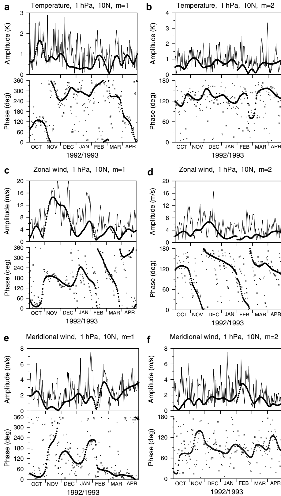
Fig. 8. Amplitudes and phases of planetary stationary (thick solid line) and planetary waves (thin lines) with zonal wave-numbers m = 1 (left column) and m = 2 (right column) for the period of October 1992–April 1993 at 10^\circ\text{N} and 1 hPa pressure level ( \sim 45 km) for the three UKMO assimilated data fields: (a and b) temperature (K); (c and d) zonal wind ( \text{ms}^{-1} ), and (e and f) meridional wind ( \text{ms}^{-1} ), respectively.
