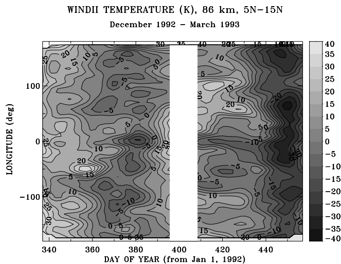
Fig. 6. Time-longitude cross section of the temperature field at 86 km from December 1 1992 to March 31, 1993, as seen by WINDII. The temperature is given as the residual between the observations and the seasonal mean.
