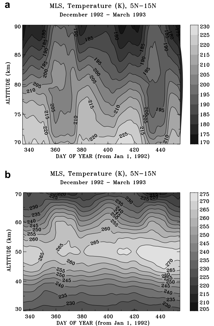
Fig. 3. Daily-mean zonal temperatures from MLS in an altitude–height section at 5^{\circ} – 15^{\circ} N and from December 1, 1992 to March 31, 1993 at: (a) 70–90 km height, and (b) 30–70 km height.
