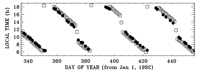
Fig. 4. Local time sampling for WINDII (solid circles) and MLS (squares) from December 1992 to March 1993 (Day 335–Day 456).
