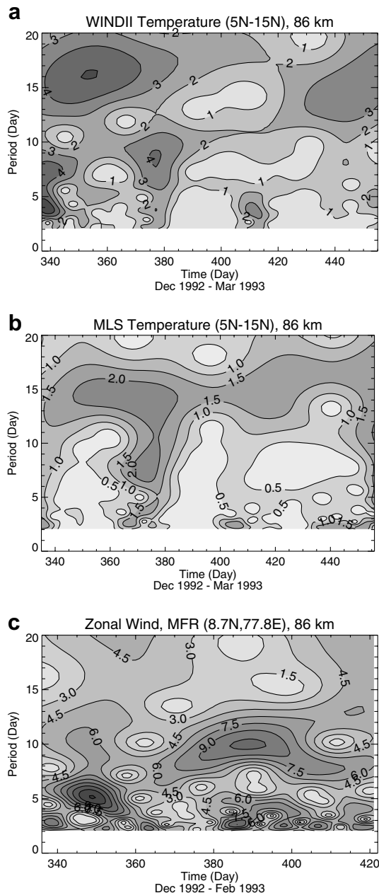
Fig. 11. Morlet wavelet at 86 km from December 1992 to March 1993 of the WINDII (a) and MLS (b) zonal mean temperatures, and from December 1992 to February 1993 of the MFR zonal winds (c) observations.
