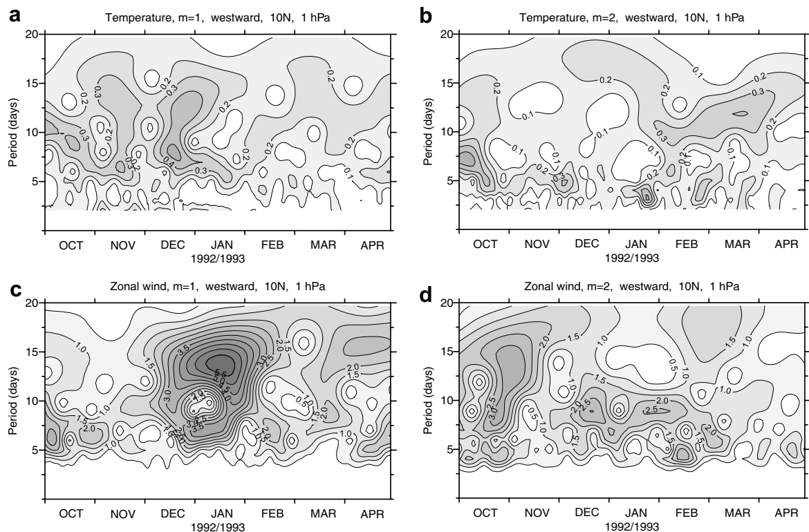
Fig. 9. Wavelet amplitude spectra at 10^\circ\text{N} and 1 hPa pressure level ( \sim 45 \text{ km} ) for planetary westward-propagating waves with zonal wave-numbers m = 1 (left column) and m = 2 (right column), for the period of October 1992–April 1993 extracted from the UKMO assimilated fields: (a and b) temperature, (c and d) zonal wind.
