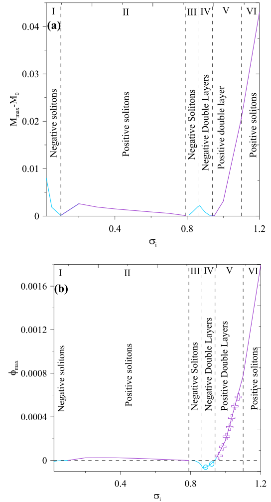
FIG. 3. Existence domain of slow ion-acoustic solitons (a) M_{max} - M_0 (b) maximum amplitude, \phi_{max} , as a function of \sigma_i for the parameters of Fig. 2. Positive solitons (regions-II and VI) and negative solitons (regions-I and III). At \sigma_i = 0.8 , slow ion-acoustic solitons ceases to exist. Double layers: negative (region-IV) and positive (region V). The circles and + signs on \phi_{max} show the existence of negative and positive double layers, respectively.
