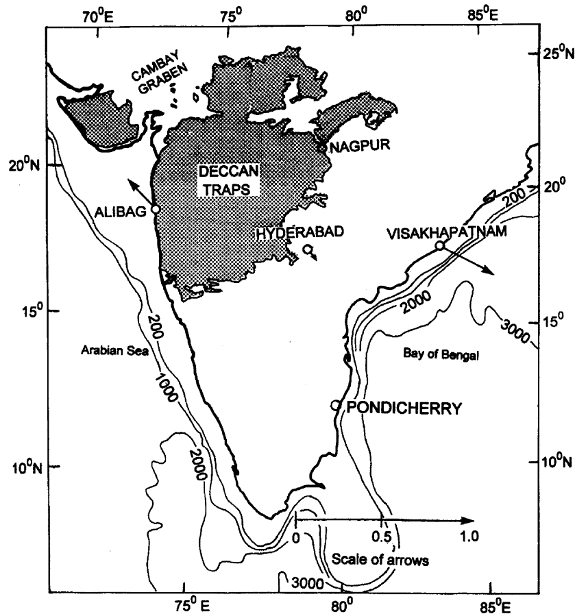
Figure 2. Map showing the locations of the three observatories, at Alibag, Hyderabad and Visakhapatnam, in peninsular India. The induction arrows corresponding to bay frequency at these stations are shown at the respective stations. Contour lines for sea water depths (bathymetry) are also shown.
