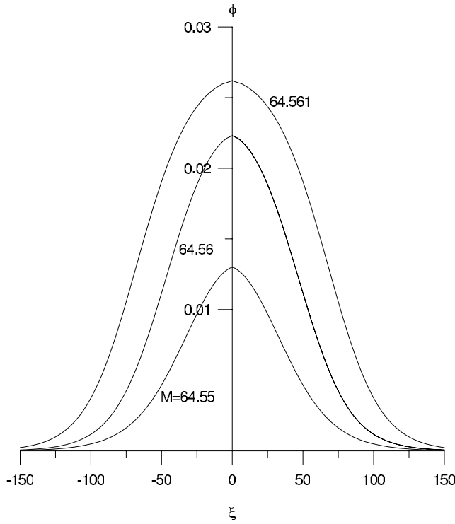
Figure 5. Potential \phi profiles for the electron-acoustic solitons for the plasma parameters of event 4, and for the Mach number M = 64.55 , 64.56 , and 64.561 .
