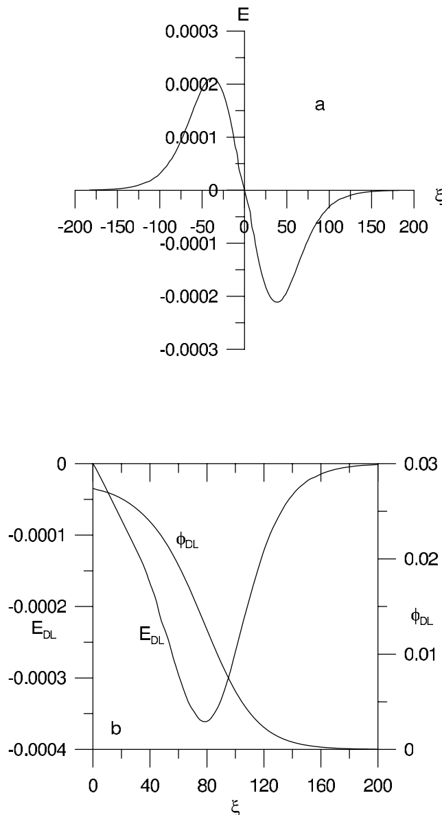
Figure 7. (a) Electric field E profile for the electron-acoustic solitons for the plasma parameters of event 4, and for M = 64.55 . The E profile has a bipolar structure. (b) Potential \phi and electric field E profiles for the electron-acoustic double layer for the plasma parameters of event 4, and for M = 64.561115 . The E profile has a monopolar structure.
