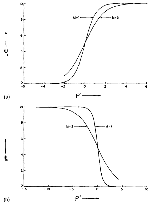
FIG. 1. Spatial potential profiles for compressive ( \psi_s ) (a) and rarefactive ( -\psi_s ) (b) shocks for typical RF dust-plasma parameters; n_{i0} \approx n_{e0} = 10^{10} \text{ cm}^{-3} , n_{D0} = 10^8 \text{ cm}^{-3} , T_e = 100 \text{ eV} , a = 10^{-5} \text{ cm} , m_D \approx 10^{-15} \text{ gm} and Q_{D0} = 10e with potential jump |\tilde{\psi}_2^{(1)} - \tilde{\psi}_1^{(1)}| \approx 10^{-3} .
