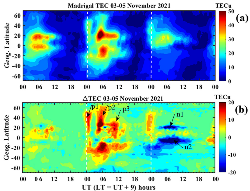
Figure 4. Shows (a) latitudinal and temporal variations of total electron content (TEC) (contour map); (b) \Delta\text{TEC} = (\text{TEC} - \text{TEC}_{\text{IQDs}} \text{ Mean}) ; \text{TEC}_{\text{IQDs}} \text{ Mean} is five international quiet days variations during the November month, over the Asian sector between 110 and 150°E longitude.
