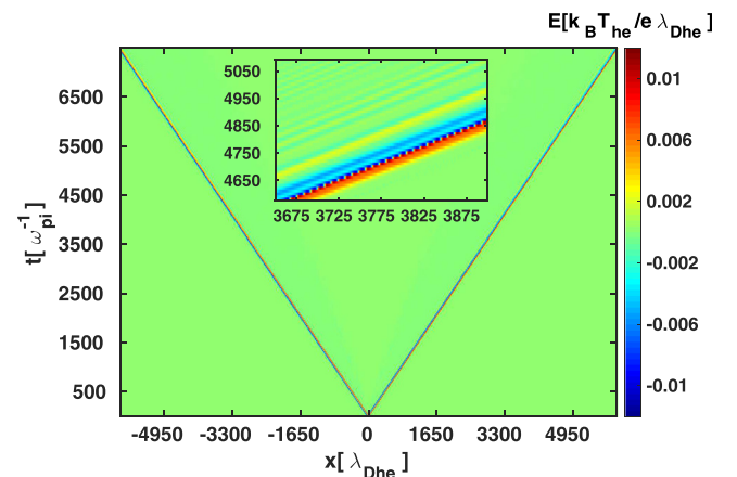
FIG. 3. Spatio-temporal evolution of the electric field in the simulation.
