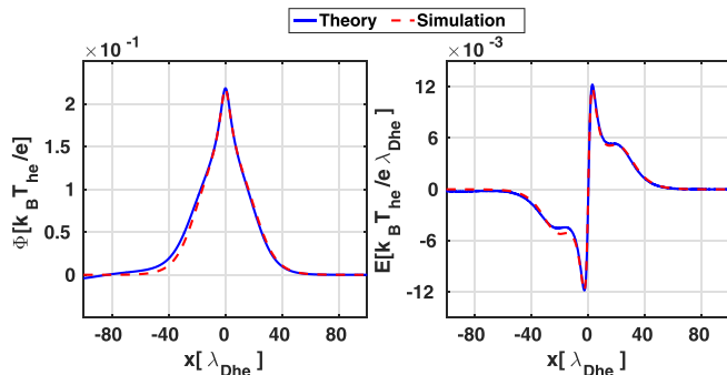
FIG. 5. The (a) potential ( \Phi ) and (b) electric field ( E_n ) profiles of the IA supersoliton from the simulation and theory.
