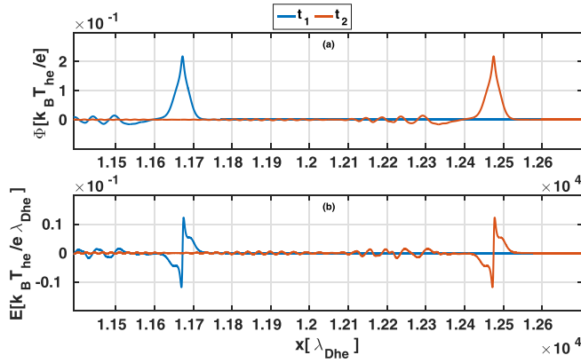
FIG. 4. Snapshots of the (a) potential and (b) electric field associated with the IA supersoliton at \omega_{pi}t_1 = 14,550 (blue curve) and \omega_{pi}t_2 = 15,550 (red curve) from the simulation.
