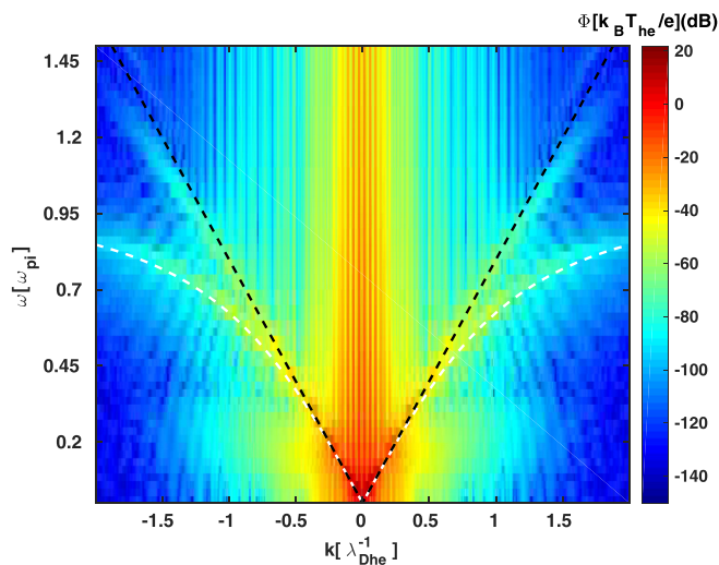
FIG. 2. \omega - k diagram during \omega_{pit}=0-200 from the simulation.
