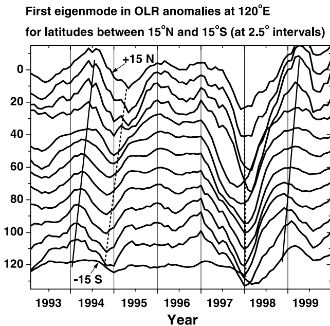
Figure 3. Temporal variation of the reconstructed OLR anomalies for latitudes between 15^{\circ}\text{N} and 15^{\circ}\text{S} at 2.5^{\circ} intervals.
