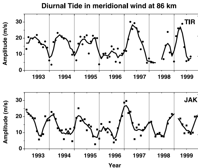
Figure 1. Monthly estimates (filled circles) of the diurnal tide in meridional wind at 86 km over Tirunelveli (TIR) (top) and Jakarta (JAK) (bottom). Continuous curves represent 3-month running means.
