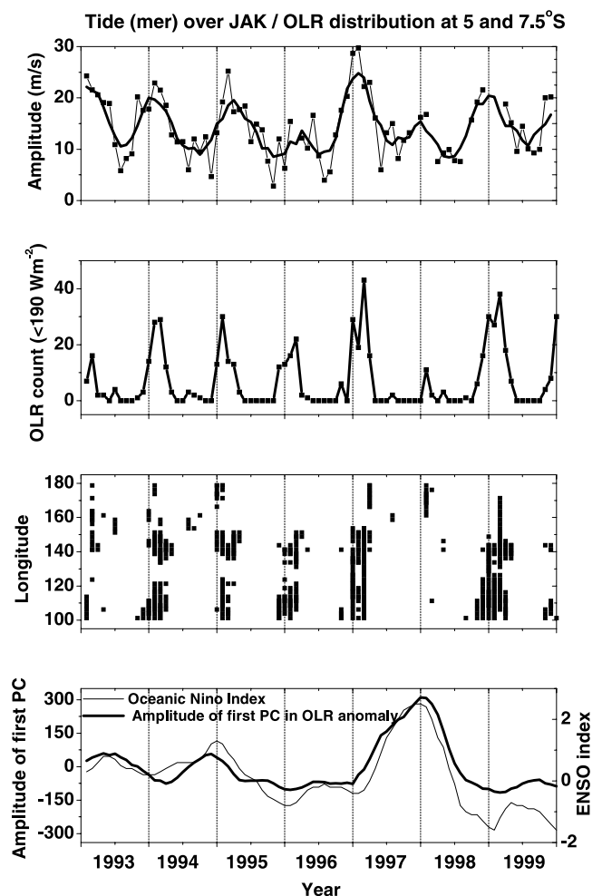
Figure 2. Temporal variation of tidal amplitude at 86 km over Jakarta (top), the OLR count (second plot) representing number of pixels on OLR maps for which the OLR brightness is less than 190 \text{ Wm}^{-2} and the position of those pixels shown as longitudinal distribution in the range 100\text{--}180^\circ\text{E} (third plot). The bottom plot depicts the Oceanic Nino Index and the amplitude of the first principal component derived from the OLR anomaly (see text for details).
