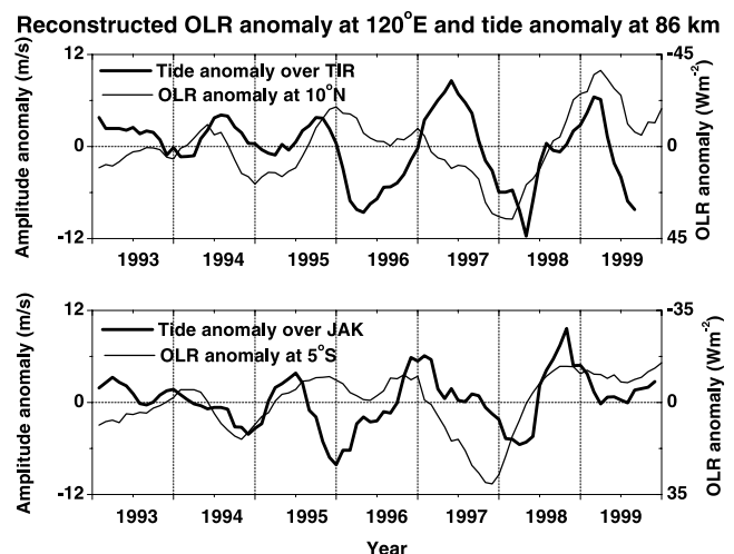
Figure 4. Comparison of tidal and reconstructed OLR anomalies at 120^{\circ}\text{E} for 10^{\circ}\text{N} /Tirunelveli (top) and 5^{\circ}\text{S} /Jakarta (bottom).
