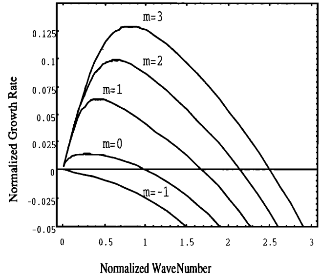
Figure 1. Normalized growth rate \gamma/\Omega_i versus normalized wavenumber kL for the tearing mode instability at the magnetopause for different values of the shear flow index m . Other parameters of the magnetopause current layer are: T_e = 25 eV, T_i = 200 eV, \rho_e = 0.34 km, and L = 100 km. For all the curves in this as well as in Figure 2, the value of the parameter \epsilon is chosen small ( \sim 0.01 or less) such that M^2 > 0 for at least |\bar{z}| \sim 3 .
