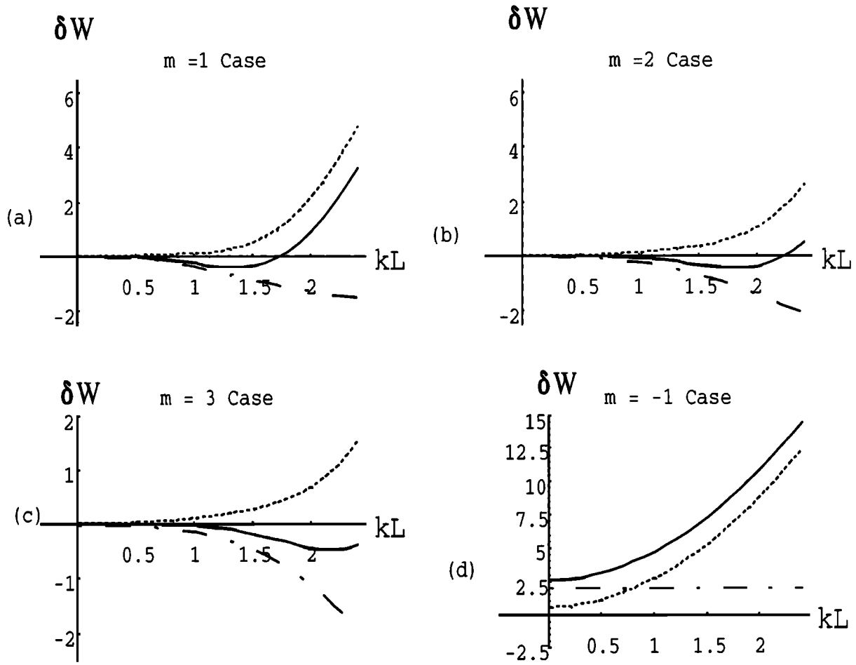
Figure 2. Variations of normalized ( \delta W_1 + \delta W_2 ) (dotted curves), \delta W_3 (dash-dot-dash curves), and \delta W = (\delta W_1 + \delta W_2 + \delta W_3) (solid curves) versus normalized wavenumbers, kL . Figures 2a–2d correspond respectively to the case of shear flow index m = 1, 2, 3 , and -1 .
