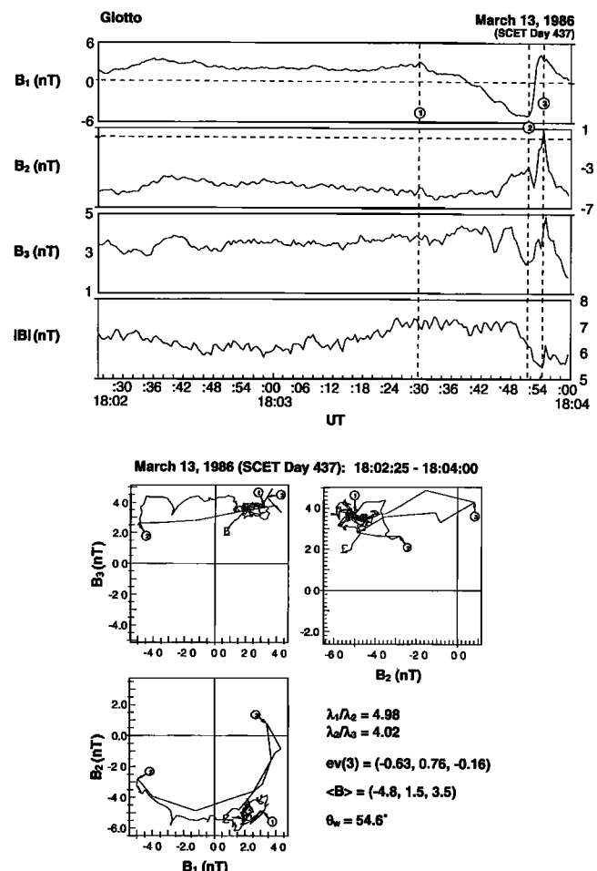
Figure 2. A Halley LF wave in minimum variance coordinates. The hodogram at the bottom indicates that the highly nonlinear wave is "arc-polarized". Most of the phase rotation occurs at the trailing portion of the interval, between points 2 and 3.
