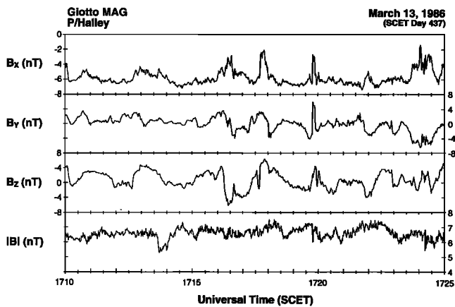
Figure 1. An example of the irregular Halley H_2O group ion cyclotron waves. Sharp temporal changes in the field components can be noted at \sim 1716 , \sim 1718 and \sim 1720 UT. The quasiperiod is \sim 120 s. There is only small compressional component associated with the fluctuations.
