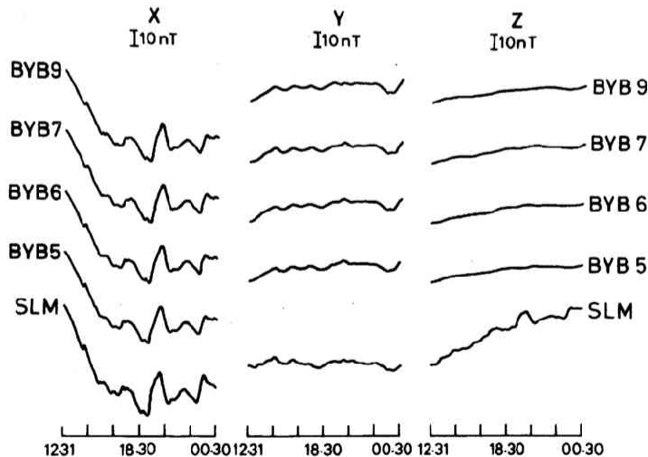
Fig. 4. Geomagnetic field variations recorded simultaneously for phase I stations corresponding to 1231-0030 Hrs (UT) of 19–20 March 1991.
