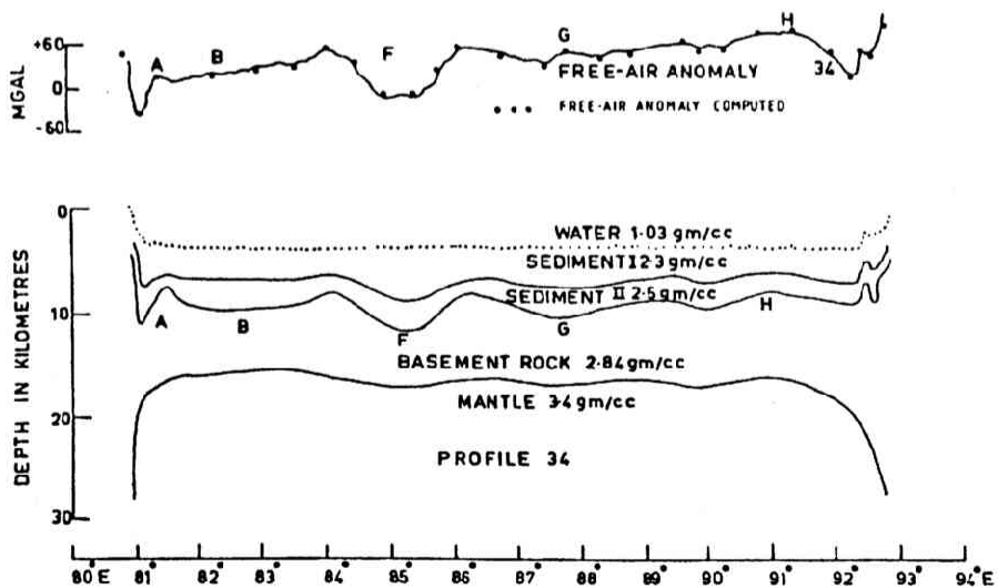
Fig. 2. Crustal structure and free air gravity anomaly observed and predicted (after Rao and Rao, 1986).
