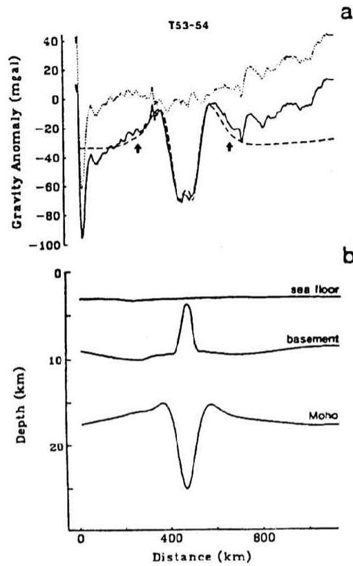
Fig. 1. (a) A comparison between the observed free air gravity anomaly (solid line), the predicted anomaly for the best model (dashed line) and residual gravity (dotted lines). (b) The "best model" (after Liu et al. , 1982).
