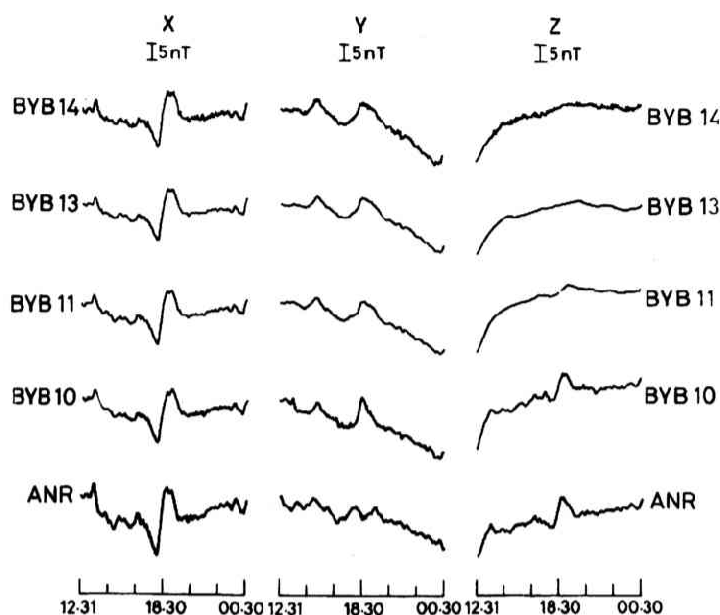
Fig. 5. Geomagnetic field variations recorded simultaneously for phase II stations corresponding to 1231-0030 Hrs (UT) of 2-3 March 1992.
