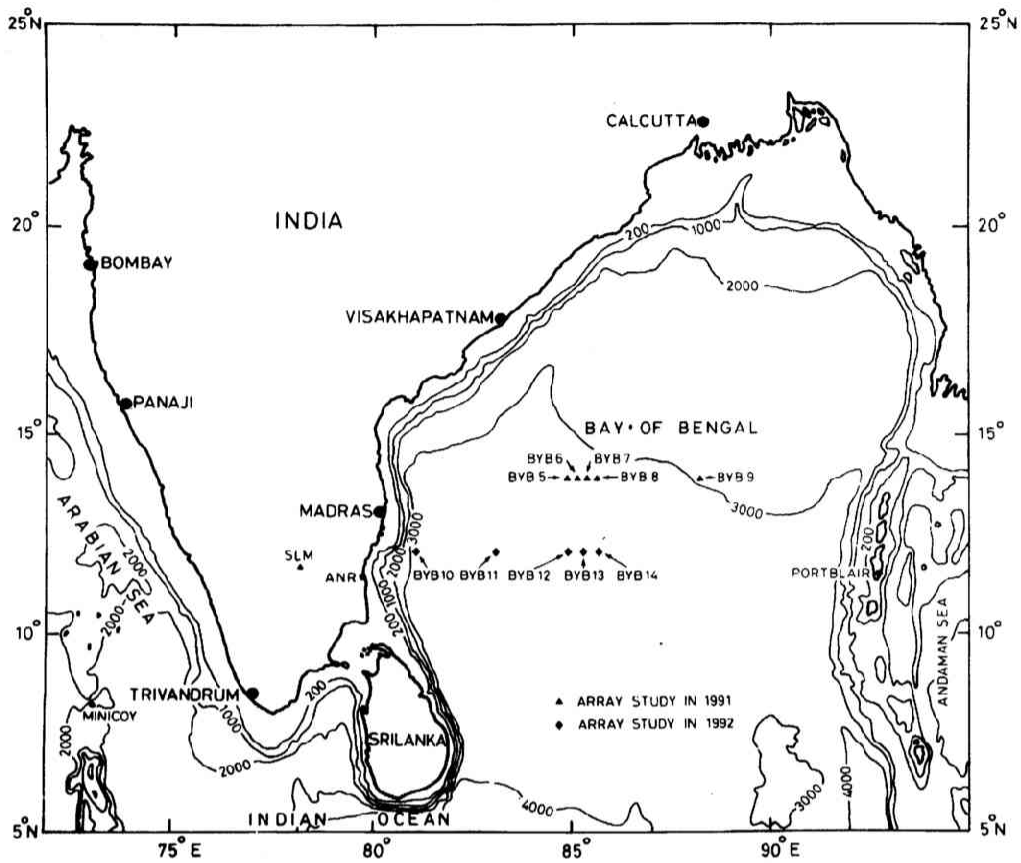
Fig. 3. Station locations with detailed bathymetry of Bay of Bengal.
