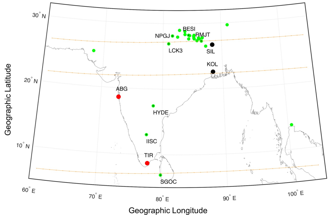
Figure 2. Network of the stations providing the data. Red dots: magnetometers; black dots: scintillations monitors; green dots: GPS stations. In green dots with a black dot inside, a subset of GPS stations used for TIDs detection and ROTI time profiles (see Figure 4). The orange lines represent the position of the dip equator and the isoclinic lines at +15°N and +20°N.
