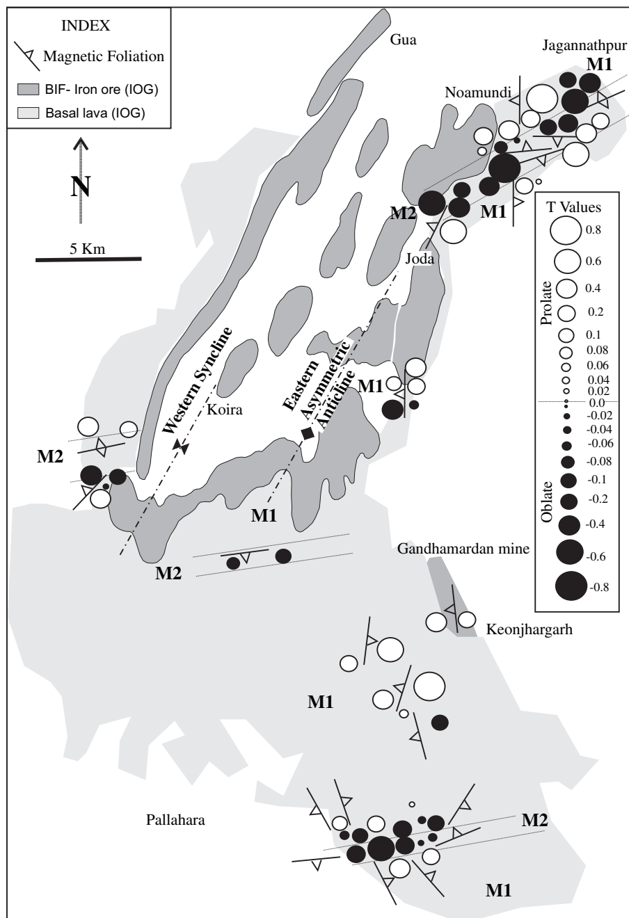
Fig. 13. Map of the 'horseshoe synclinorium' showing the mean magnetic foliation trajectory and distribution of mean values of shape parameter ( T_j ) from each sample as listed in Table 2 (similar mean T_j values for samples from a particular site are represented by a single value in the map). Note the preferential concentration of '–ve T ' values in narrow M_2 domains indicating prevalence of constrictional strain state in M_2 domains.
