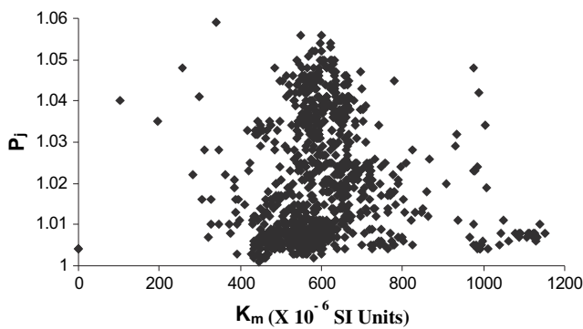
Fig. 10. Graph of degree of anisotropy ( P_j ) vs. mean bulk susceptibility ( K_m ) of 892 core specimens from 83 lava samples collected in and around the 'horseshoe synclinorium' structure, western IOG basin.
