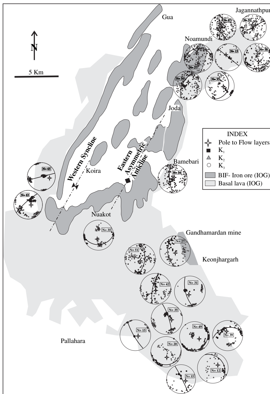
Fig. 11. Map of the 'horseshoe synclinorium' depicting the magnetic foliation trajectory in the stereographic projection diagrams of AMS directional data of all the core specimens at each site collected from lava samples as listed in Table 1 (see Fig. 1b for site locations). 'N' represents the number of core specimens at each site. The girdles in the projection diagrams represent the Magnetic foliations (F) defined by the common great circle passing through K 1 and K 2 axes of all the core specimens from samples in a single site. The pole to the 'F' is K 3 . Note that the angle between K 3 and primary layering (S 0 ) within basal lava maintains a moderate to high angle at each sample site.
