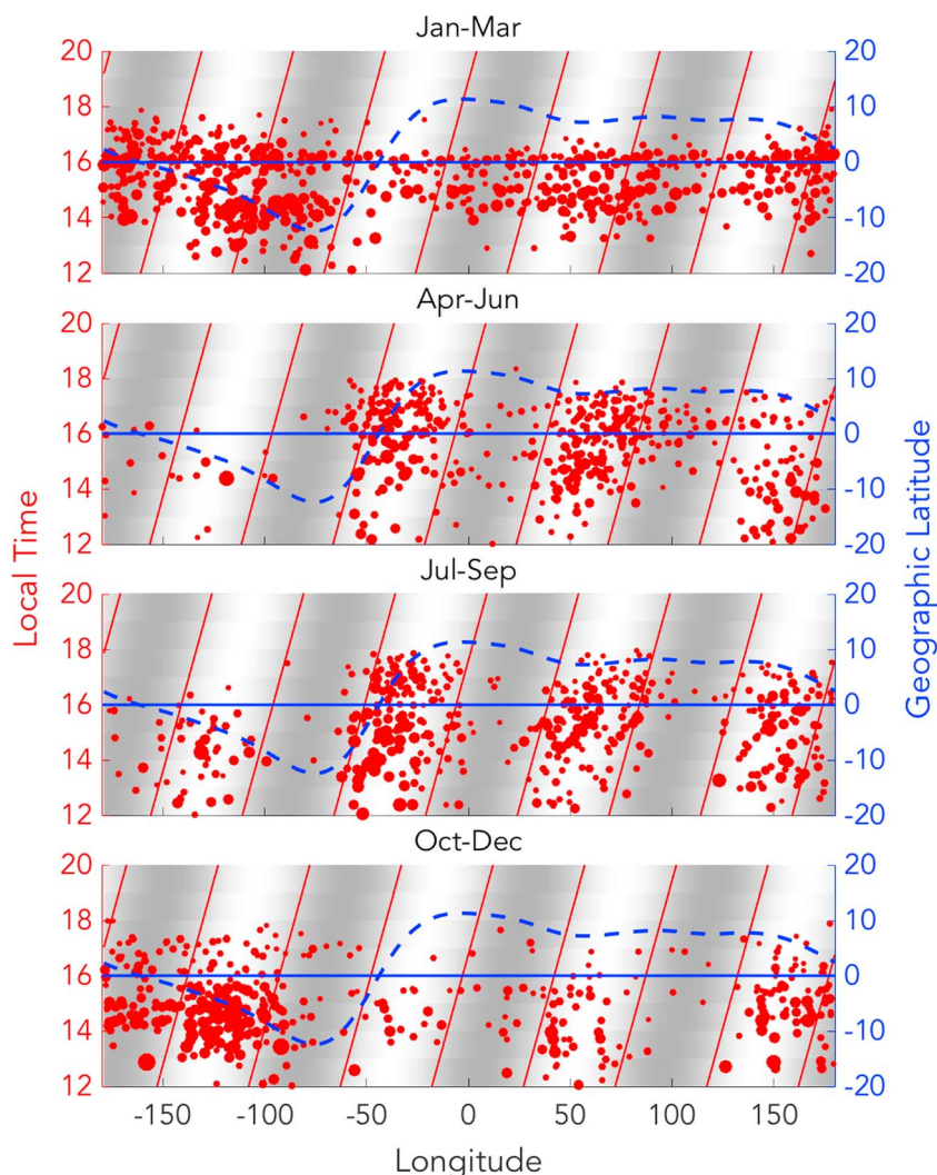
Figure 1. The afternoon counter-electrojet occurrence derived from Challenging Minisatellite Payload observations as a function of longitude and local time. The dashed line represents the dip equator as of year 2005. The vertical tilted solid lines are the DE3 zero-wind lines as derived from Thermosphere Ionosphere Mesosphere Energetics and Dynamics Doppler Interferometer observations for an altitude of 105 km. The horizontal line represents the location of the geographic equator.
