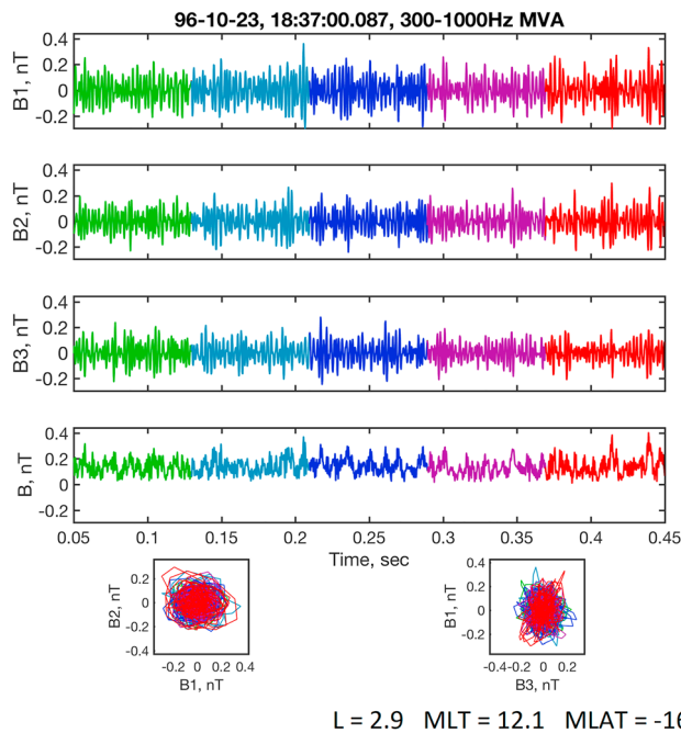
Figure 6. A \sim 0.4 -s interval that contains elliptically polarized plasmaspheric hiss. The format is the same as in Figure 4. MVA = minimum variance analysis; MLT = magnetic local time; MLAT = magnetic latitude.
