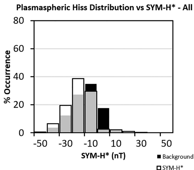
Figure 17. Same general format as in Figure 15 but for plasmaspheric hiss event interval SYM-H* values for all local time sectors. The SYM-H* plasmaspheric hiss histogram is given in white/gray with the annual background SYM-H in black. The percent occurrence scale is on the left.
