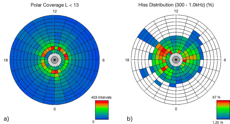
Figure 1. (a) Polar satellite coverage for the study, given as a function of L and MLT. Noon is on the top, and dawn is on the right. The coverage extends from L = 2 to L = 13 . The legend gives the number of ~2-min intervals for each \Delta L - \Delta MLT bin. (b) The plasmaspheric hiss occurrence frequencies for ~300-Hz to ~1.0-kHz waves. Each bin size is 1-hr MLT and 1 L-shell. The color code on the lower right gives the occurrence percent frequencies. MLT = magnetic local time.
