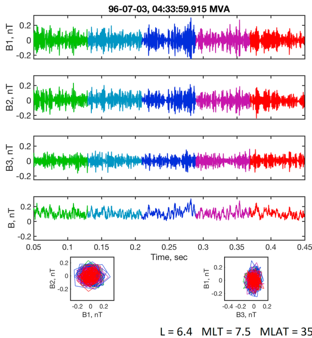
Figure 4. A \sim 0.4 -s interval with circularly polarized plasmaspheric hiss. Five different colors have been added at equal time intervals to allow the reader to follow the evolution of the waves. MVA = minimum variance analysis; MLT = magnetic local time; MLAT = magnetic latitude.
