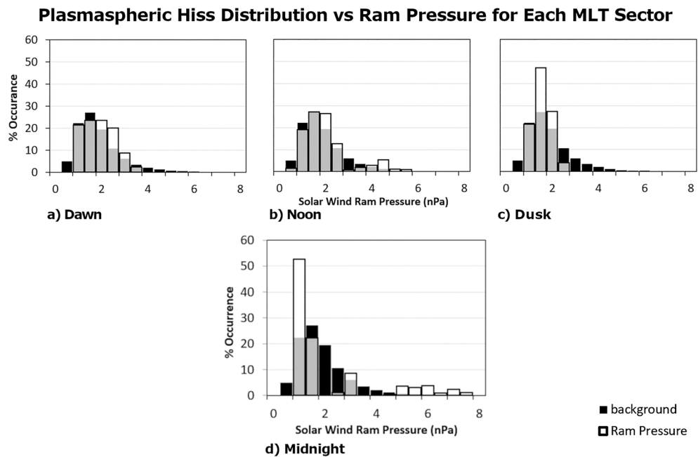
Figure 20. Same format as Figure 19 but the four local time sectors are analyzed separately. (a)–(d) correspond to the dawn, noon, dusk, and midnight sectors. MLT = magnetic local time.
