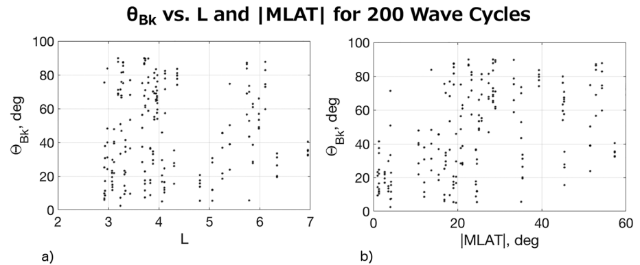
Figure 12. (a) Wave normal angle \theta_{kB} as function of L and (b) \theta_{kB} as a function of MLAT. The 200 individual wave cycles analyzed are shown in this figure. MLAT = magnetic latitude.
