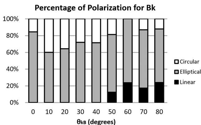
Figure 13. The percent circular, elliptically, and linearly polarized plasmaspheric hiss as a function of angle of wave k relative to the ambient magnetic field direction (B).
