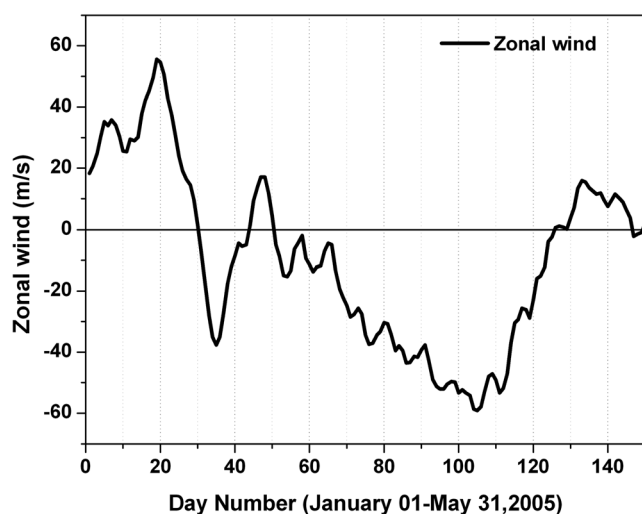
Figure 6. Day-to-day variation of daylight mean zonal wind at 88 km.
