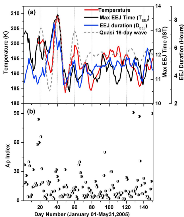
Figure 1. Time variation of daytime mesopause temperature (MT), time of the maximum equatorial electrojet (EEJ; T_{EEJ} ), and duration of the EEJ ( D_{EEJ} ) over Trivandrum.
