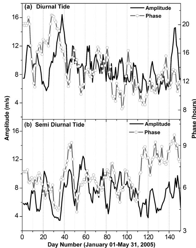
Figure 4. Time variation of the amplitude and phase of (a) diurnal and (b) semidiurnal tides in the zonal wind at 88 km.
