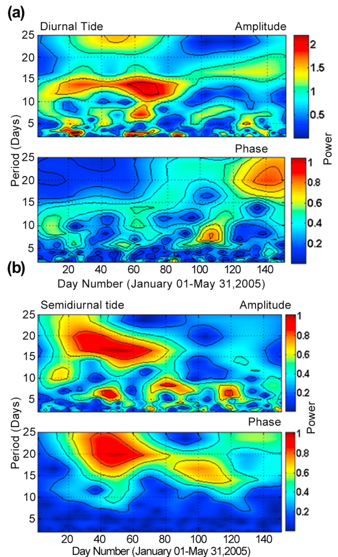
Figure 5. Wavelet periodogram for the amplitude and phase of (a) diurnal and (b) semidiurnal tides depicted in Figure 4.
