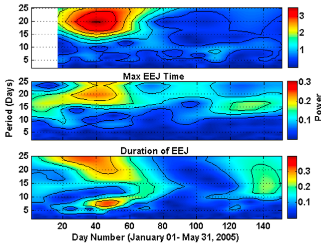
Figure 2. Wavelet periodogram for MT, D_{EEJ} , and T_{EEJ} .
