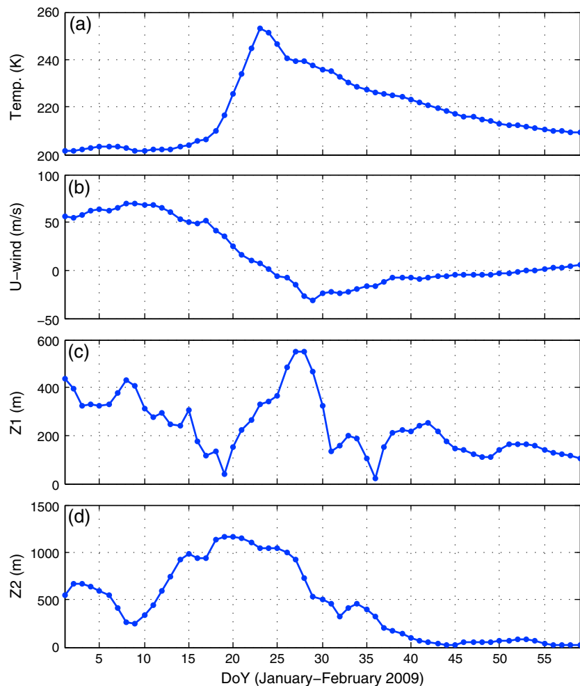
Figure 1. Temporal variation in different stratospheric parameters at 10 hPa ( \sim 30 km) over 60^{\circ} – 90^{\circ} N during January–February 2009. (a) Temperature (K) between 60^{\circ} and 90^{\circ} , (b) zonal wind at 60^{\circ} N, (c) amplitude of planetary wave 1 (Z1), and (d) amplitude of planetary wave 2 (Z2) in geopotential height at 10 hPa and 60^{\circ} N.
