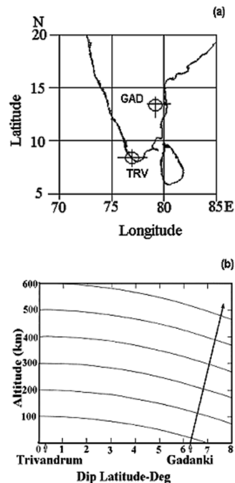
Figure 1. (a) Geographic locations and (b) magnetic field geometry for the two radar stations, Trivandrum and Gadanki.
