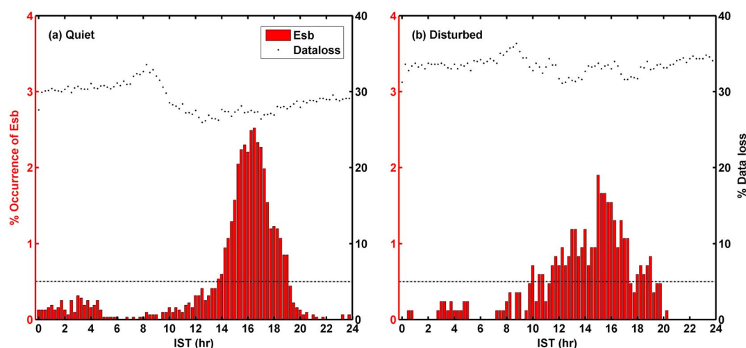
Figure 4. Percentage occurrence of Esb as a function of IST for (a) quiet and (b) disturbed days during 1996–2006. The horizontal lines indicate occurrence on 0.5% days.
