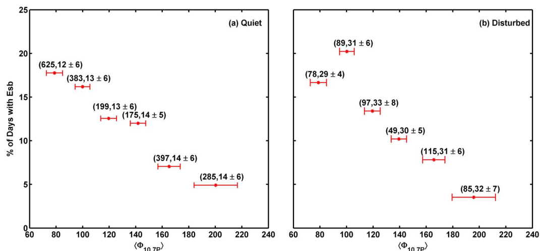
Figure 5. Percentage of days with Esb as a function of the average solar flux proxy during 1996–2006 for (a) quiet and (b) disturbed days. The numbers in parenthesis represent number of days for which ionosonde data are available and the average of daily \sum Kp , respectively, for each solar flux category. As solar activity increases, the occurrence of Esb decreases for quiet as well as disturbed days, which clearly indicates the inverse relation between the two parameters.
