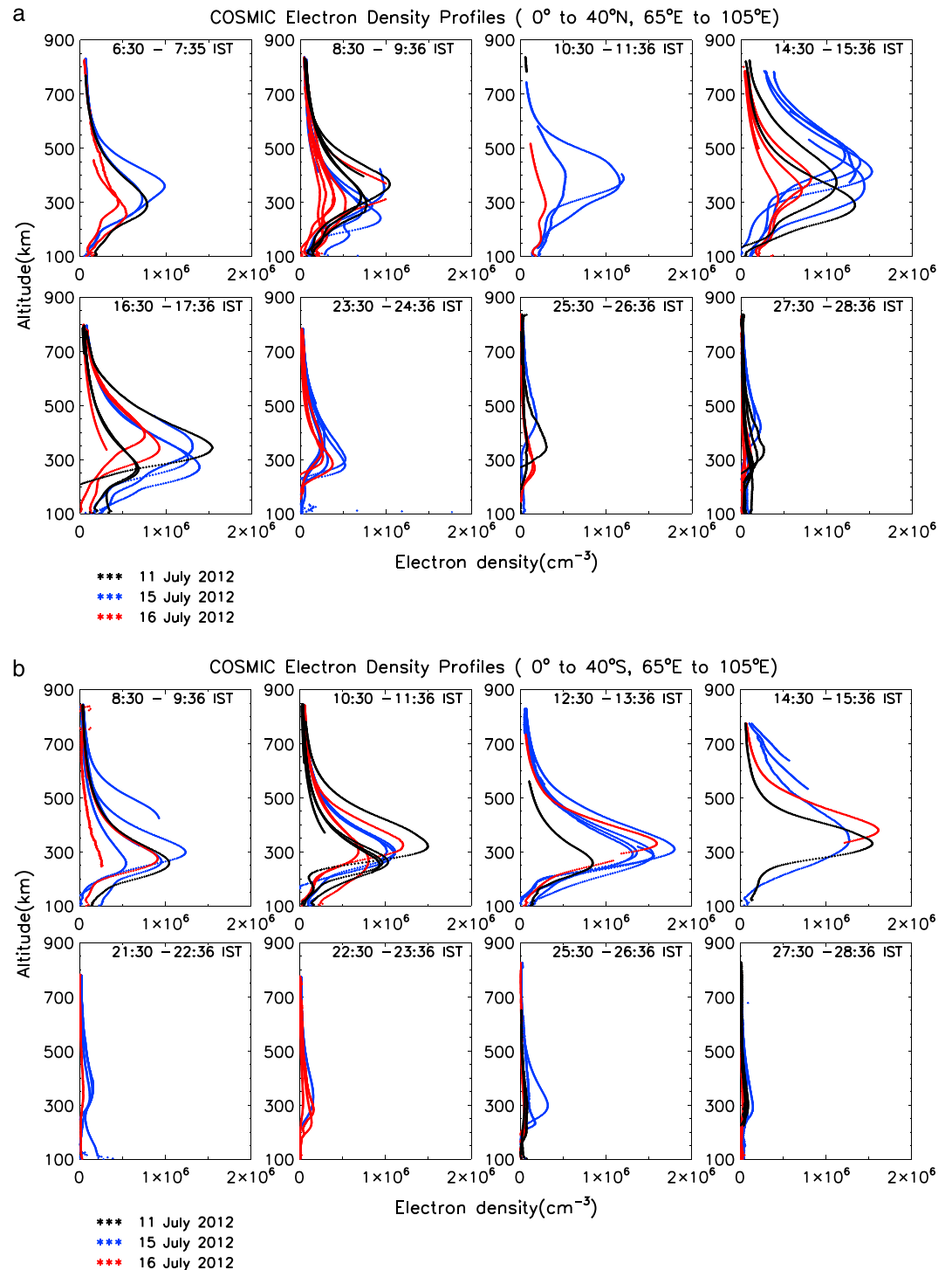
Figure 4. COSMIC RO electron density profiles obtained for different times of the day for 11 (black), 15 (blue), and 16 (red lines) July 2012, (a) for 0° to 40°N and 65° to 105°E geographical region and (b) for 0° to 40°S and 65°E to 105°E geographical region. The broadening of electron density profiles in Figure 4a during 14:30 and 15:35 IST coincides with the time of prompt penetration electric field on 15 July. On 16 July, the ionospheric density profiles were completely suppressed on most of the hours in the daytime in the Northern Hemisphere. The electron density variations in the Southern Hemisphere (Figure 4b) did not show any significant variations except for high-density values during 14:30 to 15:35 IST on 16 July.
