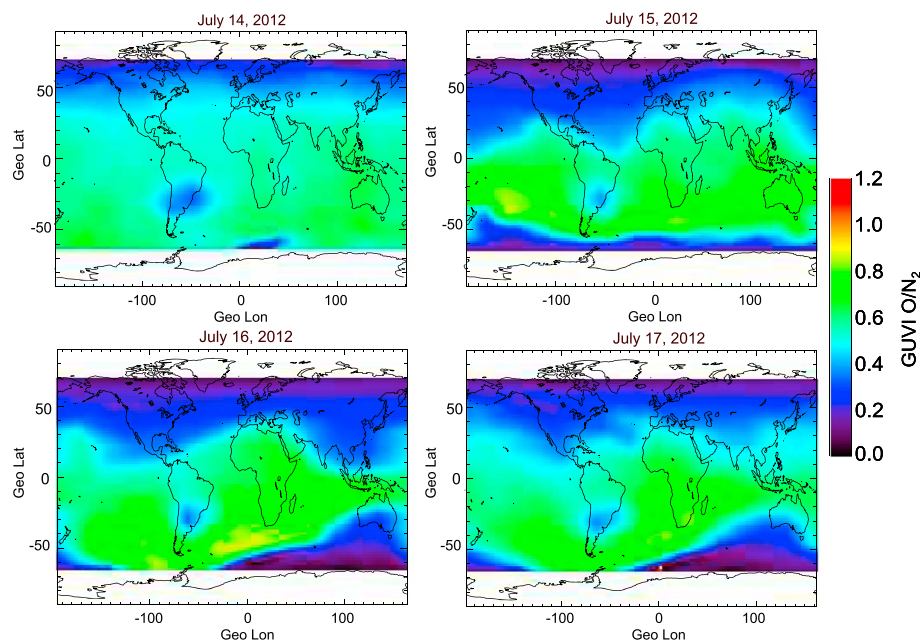
Figure 7. TIMED/GUVI maps of [O/N_2] during 14–17 July 2012. Thermospheric neutral compositional variations in terms of [O/N_2] showed enhancements in atomic oxygen over low latitudes on 15 July while strong depletion in [O/N_2] on 16 July supports the enhancement of molecular nitrogen mainly over the Northern Hemispheric low latitudes. Gradual recovery was observed in [O/N_2] on 17 July.
