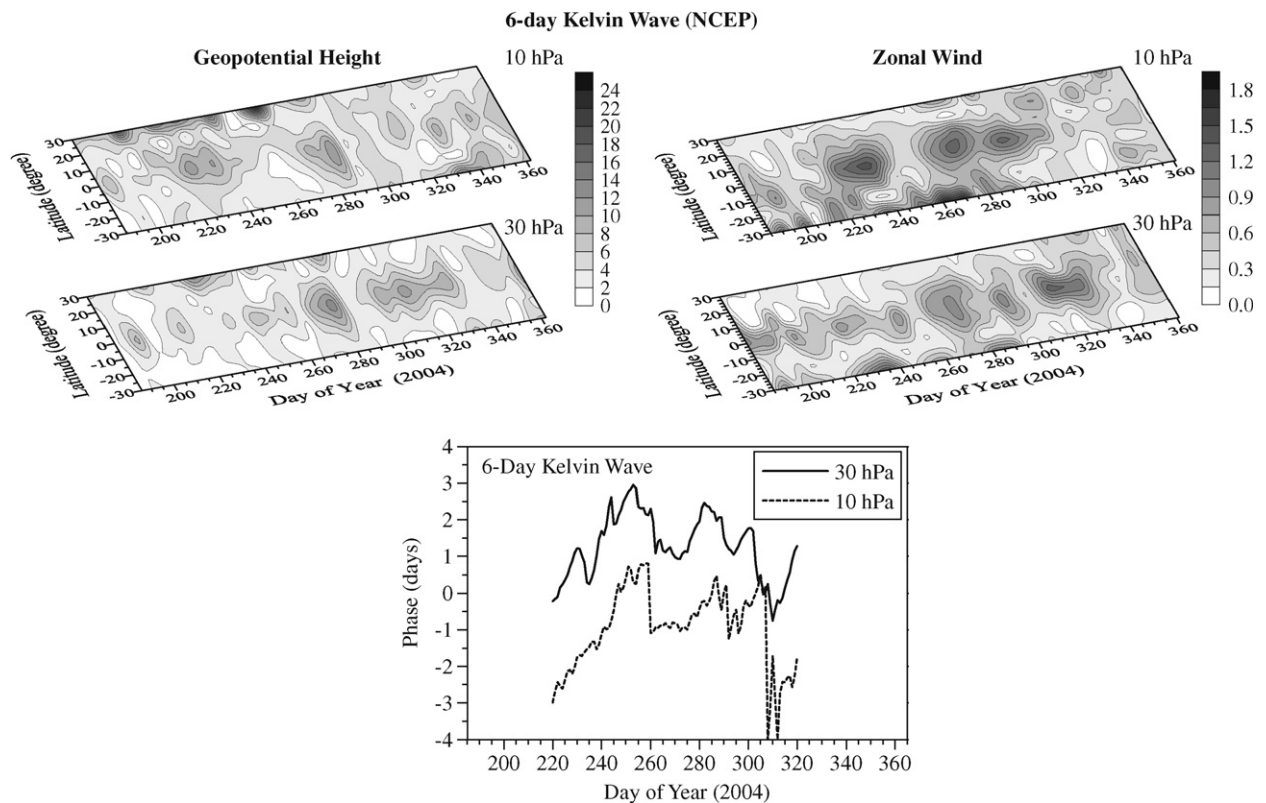
Fig. 2. Latitude–time cross-sections of the \sim 6 -day Kelvin E1 wave amplitudes at 30 and 10 hPa extracted from the geopotential height data (left upper row plot) and from the zonal wind data (right upper row plot); the bottom plot shows the phases of the \sim 6 -day Kelvin wave in the zonal wind at 30 hPa (solid line) and 10 hPa (dash line); the waves are extracted in the latitudinal range ( 30^\circ\text{N} – 30^\circ\text{S} ).
