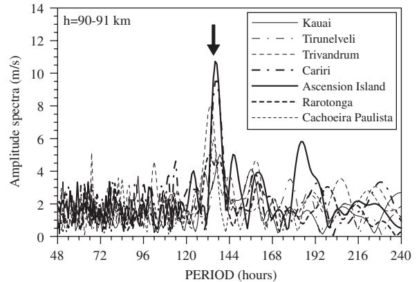
Fig. 7. Amplitude spectra of the zonal wind at 90–91 km height calculated for periods between 2 and 10 days for all stations; the arrow shows the predominant period.
