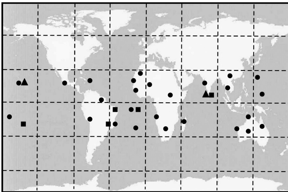
Fig. 4. A map showing the locations of MLT radars (meteor radars are marked by squares, while the MF radars by triangles) and magnetometer stations (marked by full circles).
