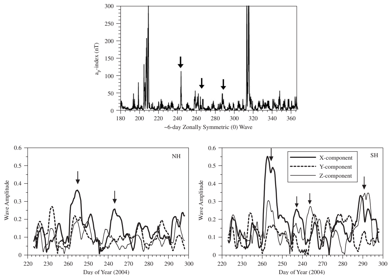
Fig. 15. The 3-hourly geomagnetic a_p -index (upper plot) and the amplitudes of the \sim 6 -day zonally symmetric (0) wave observed in the X- (tick solid line), Y- (tick dash line) and Z-components (thin solid line) for the NH (left bottom plot) and for the SH (right bottom plot).
