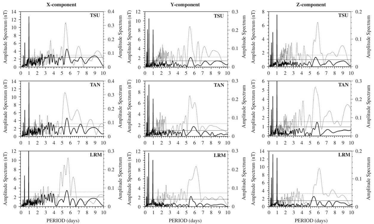
Fig. 13. Same as Fig. 12 but for stations in the SH.
