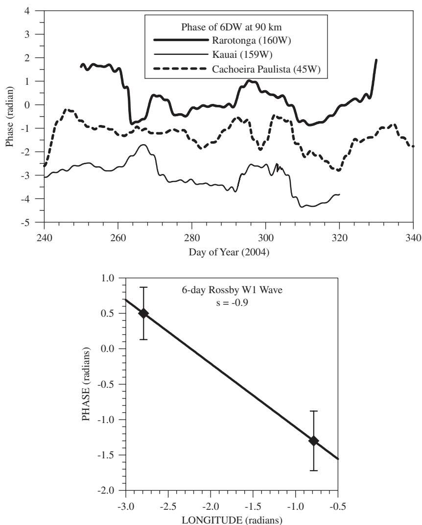
Fig. 10. The instantaneous phases of the \sim 6 -day wave at three tropical stations for 90 km height obtained by complex demodulation (upper plot); phase slope of the \sim 6 -day wave observed in the tropical MLT region.
