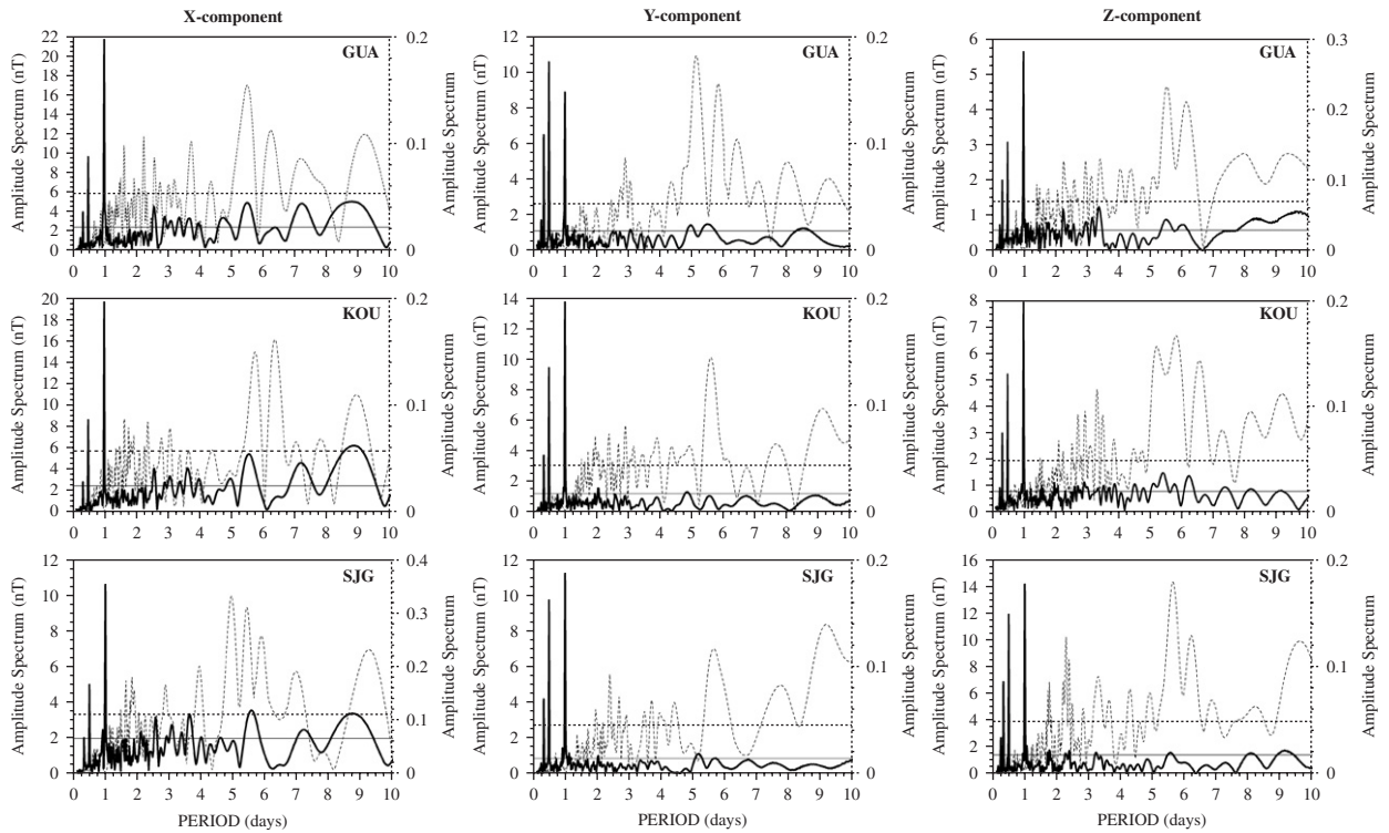
Fig. 12. Amplitude spectra in the period interval 0.25–10 days calculated from the raw (solid line) and analysed (dash line) geomagnetic data of three magnetometer stations in the NH.
