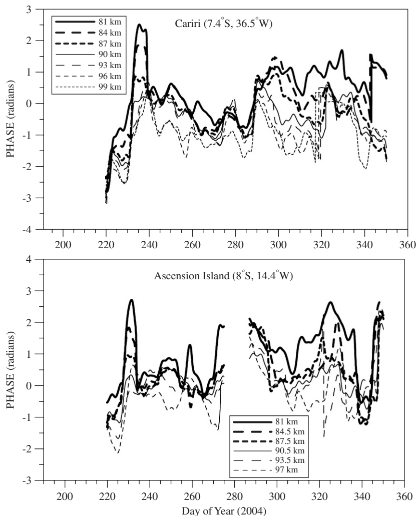
Fig. 9. The instantaneous phases of the \sim 6 -day wave for all heights at Cariri (upper plot) and Ascension Island (bottom plot) obtained by complex demodulation.
