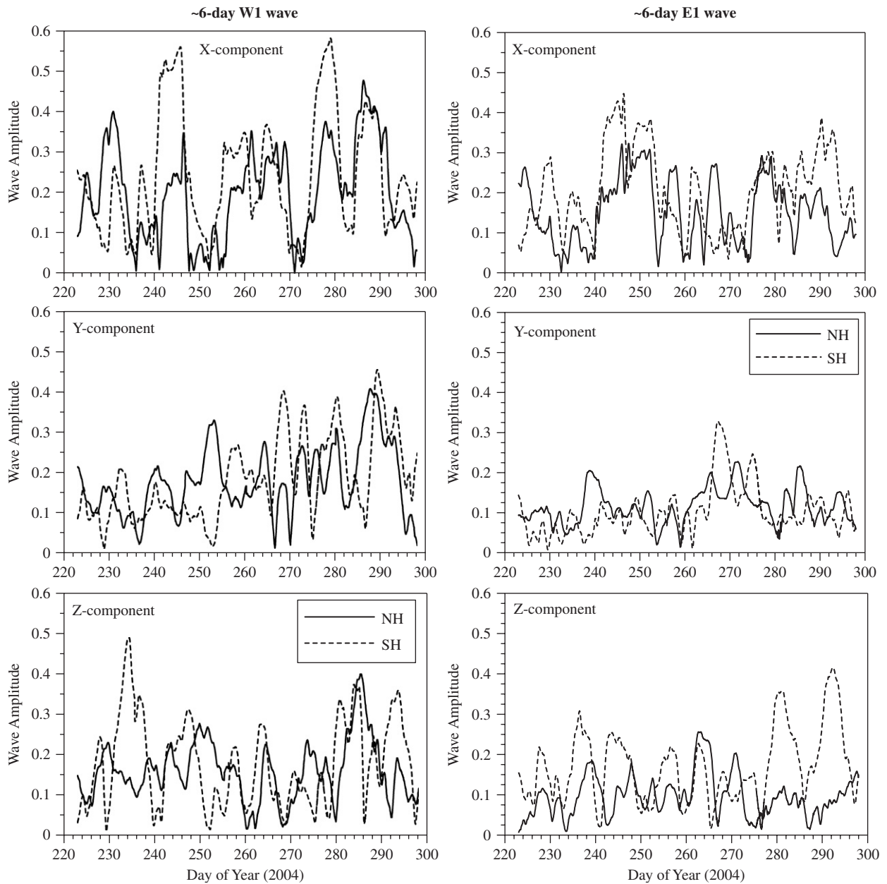
Fig. 14. Amplitudes of the ~6-day W1 (left column of plots) and ~6-day E1 (right column of plots) waves observed in the X- (upper row of plots), Y- (middle row of plots) and Z-components (bottom row of plots) for the NH (solid line) and SH (dash line).
