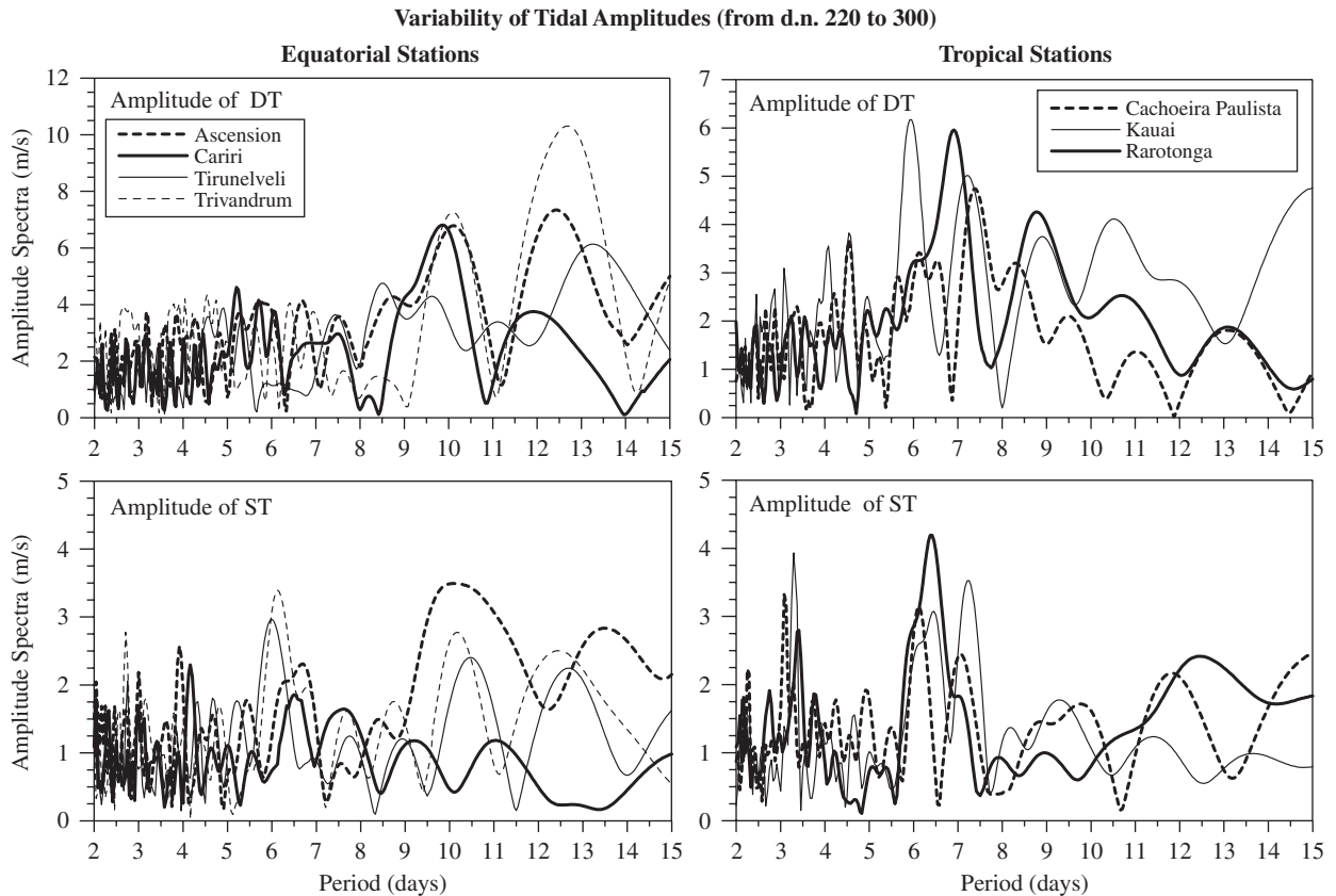
Fig. 16. Spectra of the 24-h (upper row of plots) and 12-h tidal amplitudes (bottom row of plots) for the equatorial (left column of plots) and tropical (right column of plots) MLT region.
