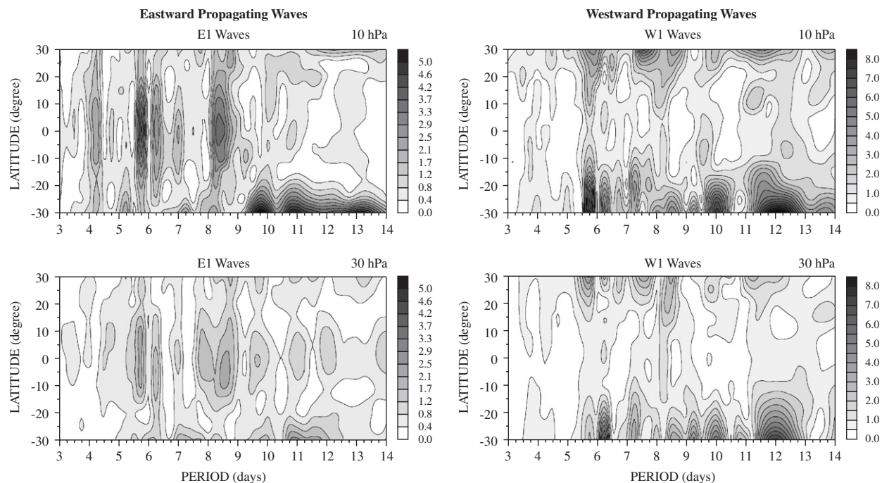
Fig. 1. Latitudinal spectra for the eastward (left column of plots) and westward (right column of plots) travelling waves with zonal wavenumber 1 for geopotential levels at 30 hPa (bottom row of plots) and at 10 hPa (upper row of plots).
