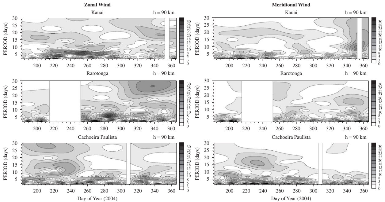
Fig. 6. Same as Fig. 5 but for the tropical stations: Kauai, Rarotonga and Cachoeira Paulista.
