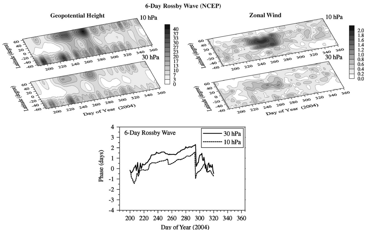
Fig. 3. Latitude–time cross-sections of the \sim 6 -day Rossby W1 wave amplitudes at 30 and 10 hPa extracted from the geopotential height data (left upper row plot) and from the zonal wind data (right upper row plot); the bottom plot shows the phases of the \sim 6 -day Rossby wave in the zonal wind at 30 hPa (solid line) and 10 hPa (dash line); the waves are extracted in the latitudinal range ( 60^\circ\text{N} – 60^\circ\text{S} ).
