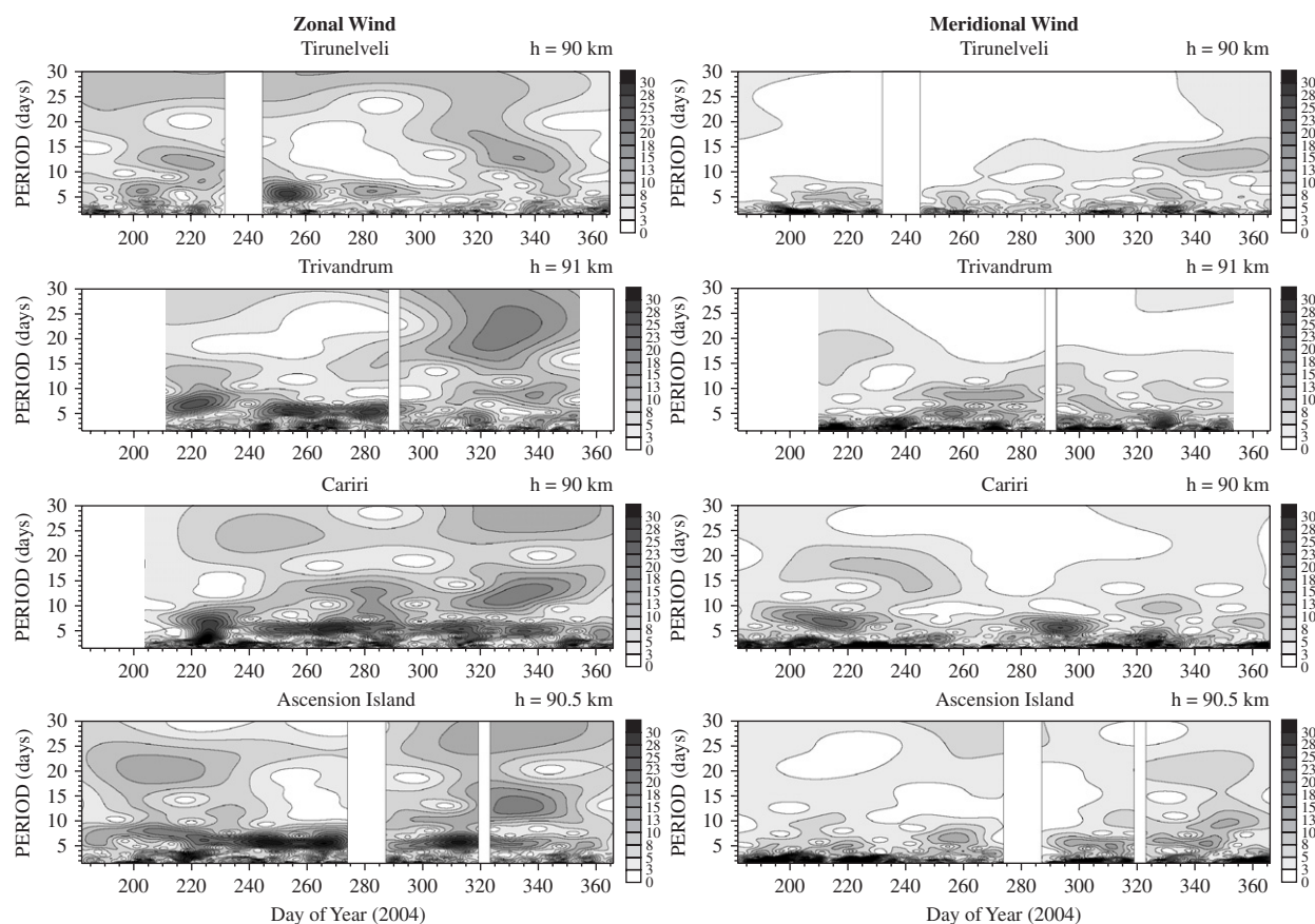
Fig. 5. Wavelet spectra of the zonal (left column of plots) and meridional (right column of plots) winds at 90–91 km height calculated for periods between 2 and 30 days for the equatorial stations: Tirunelveli, Trivandrum, Cariri and Ascension Island.
