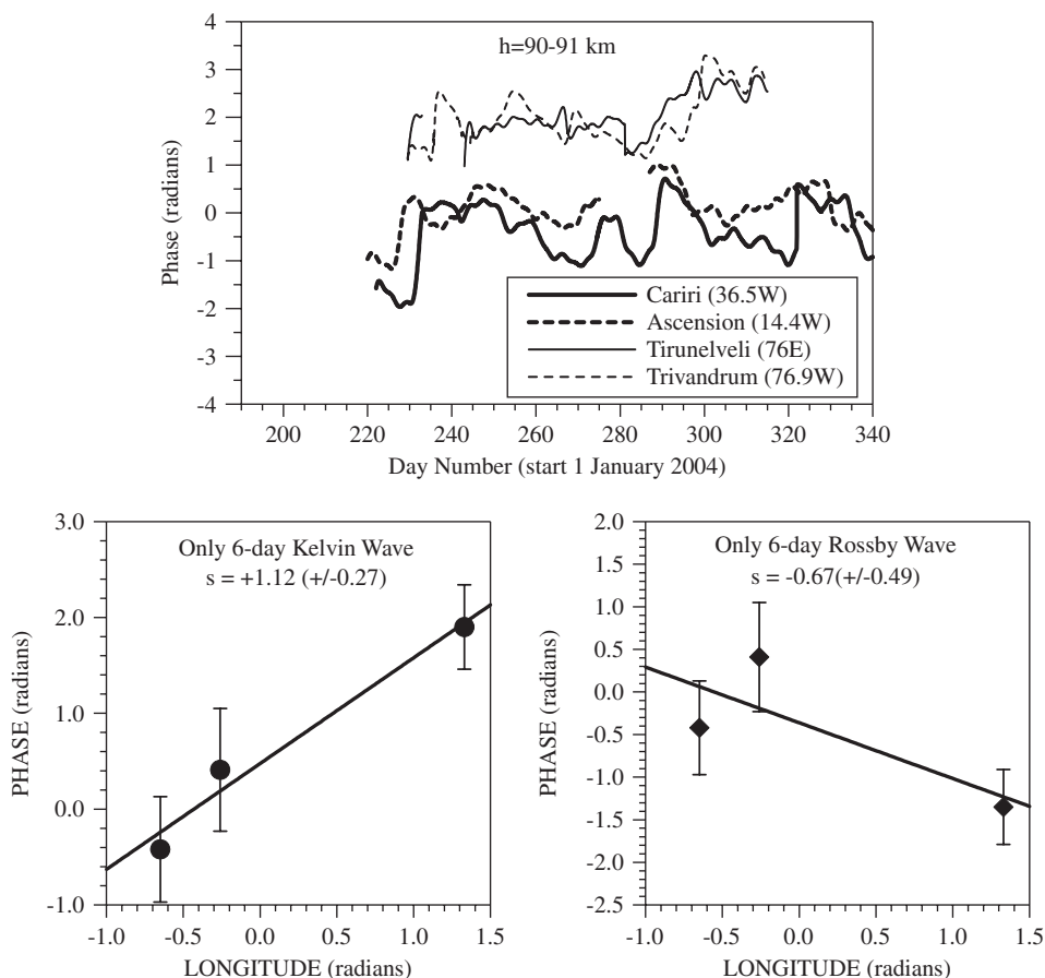
Fig. 8. The instantaneous phases of the \sim 6 -day wave at four equatorial stations for 90–91 km height obtained by complex demodulation (upper plot); phase slope of the \sim 6 -day wave assuming that it belongs to Kelvin type of waves (left bottom plot), and phase slope of the \sim 6 -day wave assuming that it belongs to Rossby type of waves (right bottom plot).
