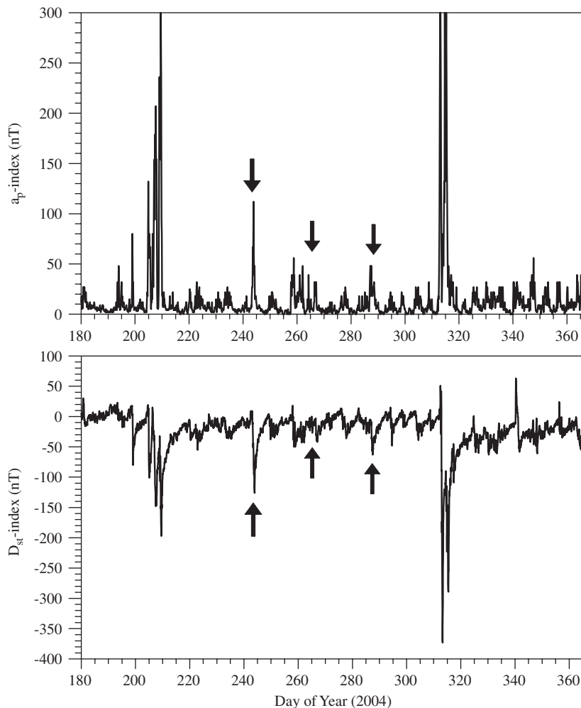
Fig. 11. The 3-hourly geomagnetic a_p -index (upper plot) and the hourly equatorial D_{st} -index (bottom plot) for the period of July–December 2004; the arrows mark the moderate/weak geomagnetic disturbances between days 220 and 300.
