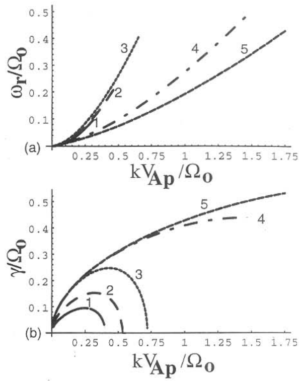
Figure 2. Variation of normalized real frequency \omega_r/\Omega_o (a), and growth rate \gamma/\Omega_o (b) versus normalized wavenumber kV_{Ap}/\Omega_o for the helicon mode instability driven by O^+ ions in the CPS region for A_e = A_p = 0 , and A_o = 2.0 . For the curves 1, 2, and 3, R = 1.0 , and M = 0.05, 0.1 , and 0.2 , respectively. For the curves 4 and 5, M = 0.2 , and R = 5.0 and 10.0 , respectively.
