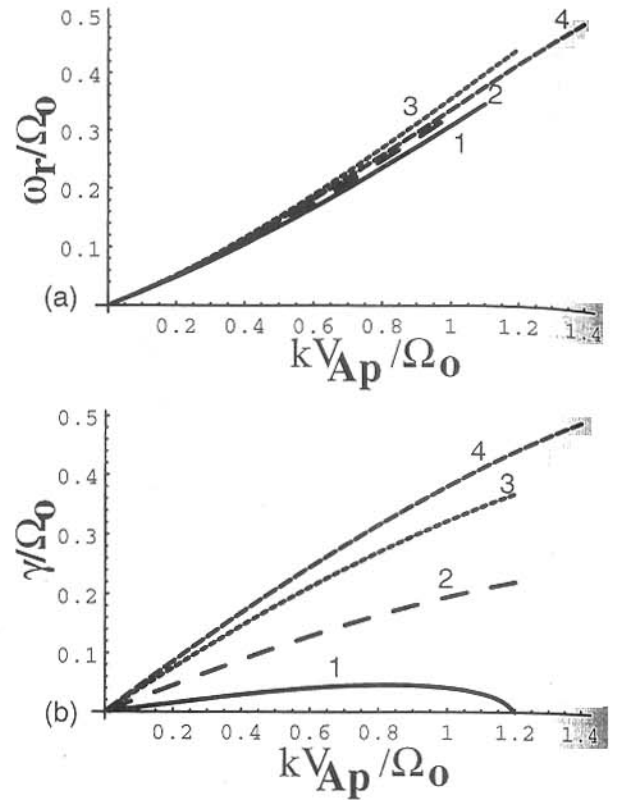
Figure 3. Variation of normalized real frequency \omega_r/\Omega_o (a), and growth rate \gamma/\Omega_o (b) versus normalized wavenumber kV_{Ap}/\Omega_o for the RH mode (helicon) instability driven by O^+ ions in the CPS region for A_p = 0 , M = 0.25 , and R = 10.0 . For the curves 1, 2, and 3, A_p = 0.0 , and A_o = 2.0, 3 , and 5 , respectively. For curve 4, A_o = 5 and A_p = 1.0 . Note that LH mode is also excited for parameters considered here as well as in Figure 4. However, the growth rates of the LH modes are smaller than the RH modes and hence not shown.
