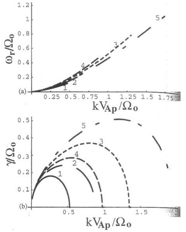
Figure 1. (a) Variation of normalized real frequency \omega_r/\Omega_o , (b) and growth rate \gamma/\Omega_o versus normalized wavenumber kV_{Ap}/\Omega_o for the helicon mode instability driven by O^+ ions in the CPS region for M = U_o/V_{Ap} = 0.25 , R = \rho_o/\rho_p = 2.0 , A_e = 0 , and \beta_{\parallel o} = 3.5 . The curves 1, 2, 3, and 4 are for A_p = 0 , and A_o = (\beta_{\parallel o} - \beta_{\perp o}) = 0.1, 0.5, 1.0 , and 2.0 , respectively. The curve 4 and 5 are for A_o = 2.0 and A_p = -0.5 and 0.5 respectively. For the parameters considered here as well as in Figures 2, the LH mode instability does not exist.
