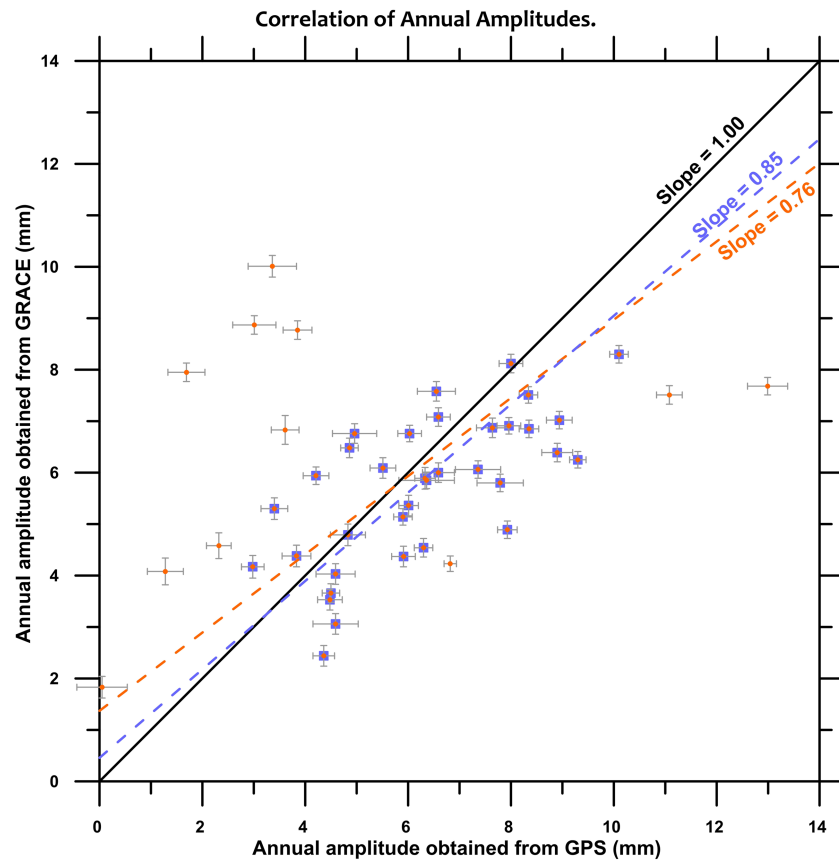
Figure 4. Correlation between annual amplitude estimated from the seasonal signals observed in GPS and GRACE measurements. The black continuous line shows the ideal condition in which GPS and GRACE perfectly match each other (slope = 1). The orange dash line indicates the estimated best fit line to the GPS and GRACE data for the entire GPS network (orange color data points). The blue dash line indicates the estimated best fit line to the GPS and GRACE data for GPS sites in Nepal and NW Himalaya for the comparison of result with Fu and Freymueller (2012) (orange data points with blue square).
