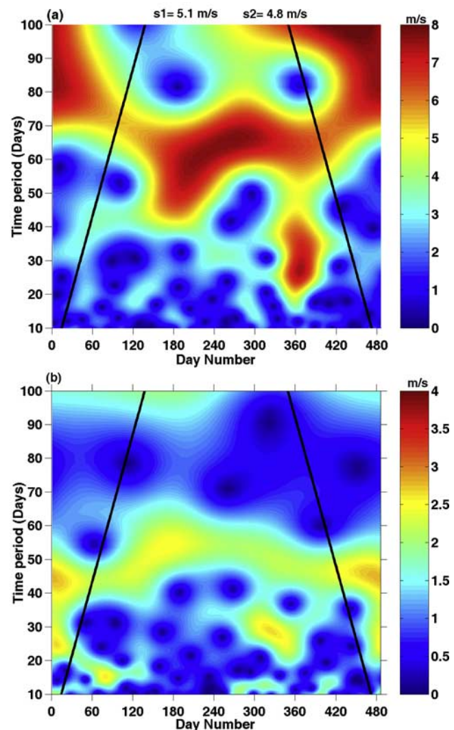
Figure 2. Wavelet spectra of (a) zonal and (b) meridional wind at 84 km ( s_1 and s_2 indicate the 95% confidence level amplitudes for 50- to 70- and 20- to 40-day oscillations, respectively).
